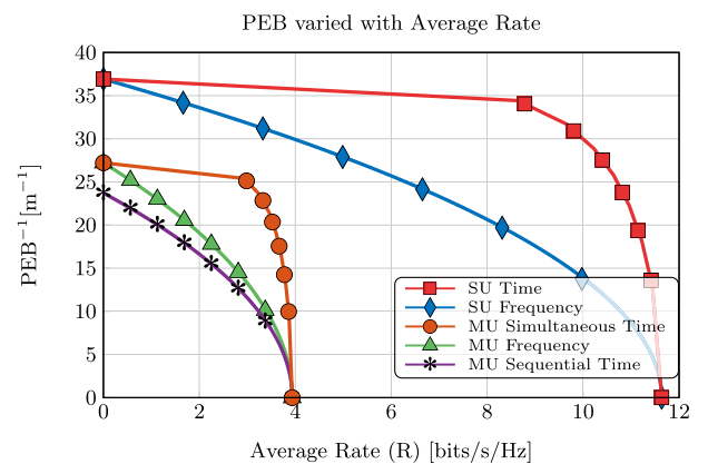
FIGURE 12. PEB vs. average rate trade-off for both time and frequency division strategies among the 3 users.
