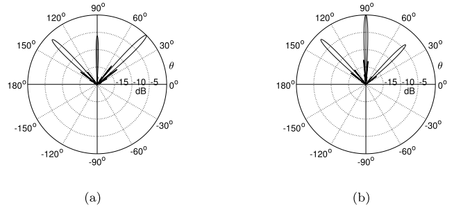
FIGURE 6. Example of normalized beam direction for a localization-optimized beamformer in the multi-user case, according to (a) min max and (b) proportional fairness strategies.
