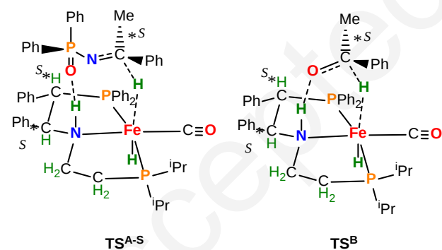
Figure 1. The proposed transition state structure ( \text{TS}^{\text{A-S}} ) for the transfer of a hydride from the dihydride complex to the activated N -phos- phinoylimine 2a compared with that to acetophenone ( \text{TS}^{\text{B}} ) to give the ( S ) imine or alcohol, respectively.
