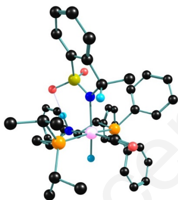
Figure 4. Structure of the amido complex 16 , with the amide form of ( S )-amine 5b coordinated to [\text{FeH}(\text{CO})(\text{P}-\text{NH}-\text{P}')^+] . Non-essential hydrogens have been deleted for the sake of clarity.
