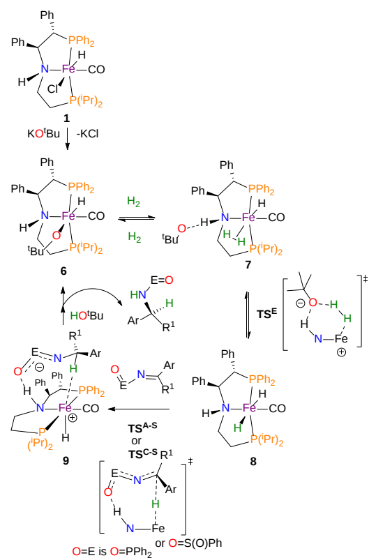
Scheme 1. Proposed Catalytic Cycle for the Asymmetric Imine Hydrogenation Catalyzed by an Iron P-NH-P' Complex.
