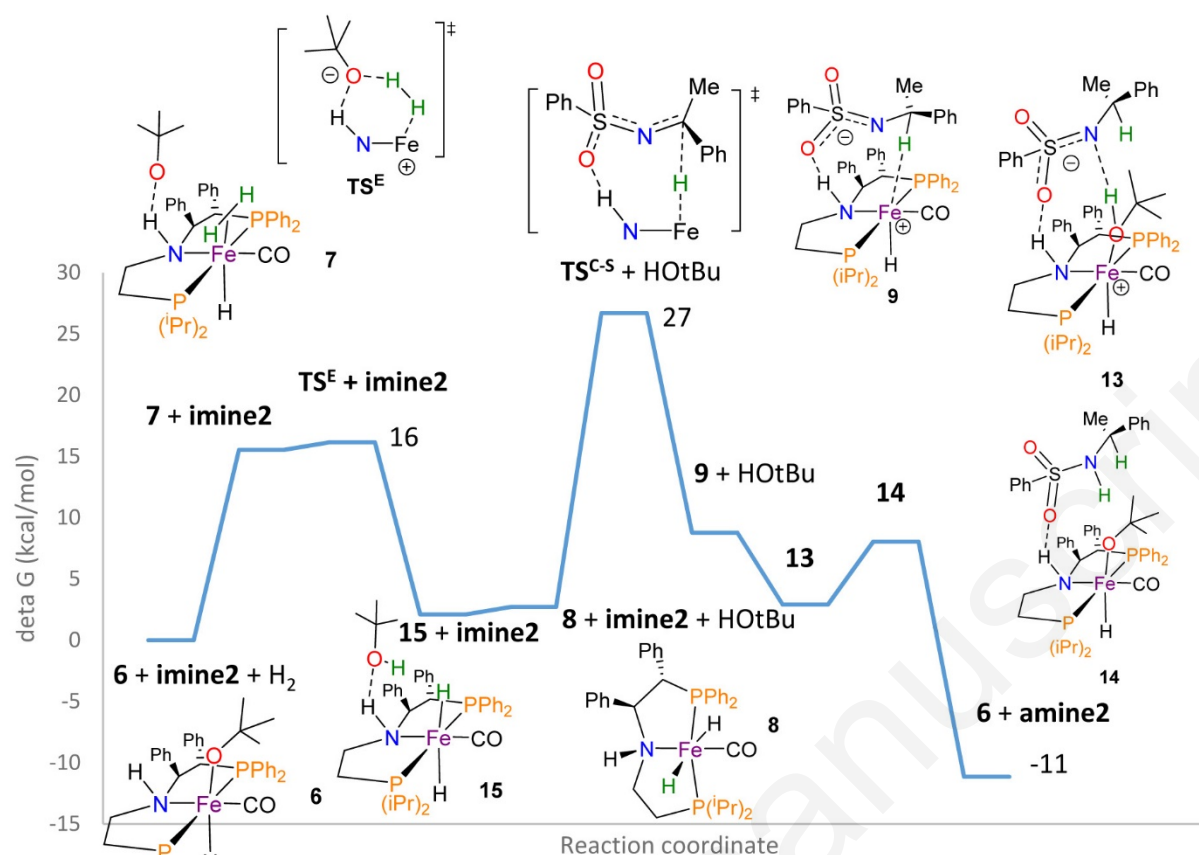
Figure 3. Reaction coordinate diagram corresponding to the catalytic cycle shown in Scheme 2.
