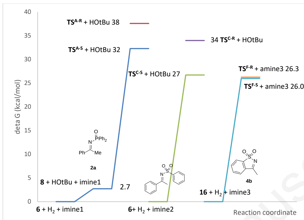
Figure 6. The energy span of the catalysis for three imines, representing also the enantiodetermining hydride transfer transition state.
