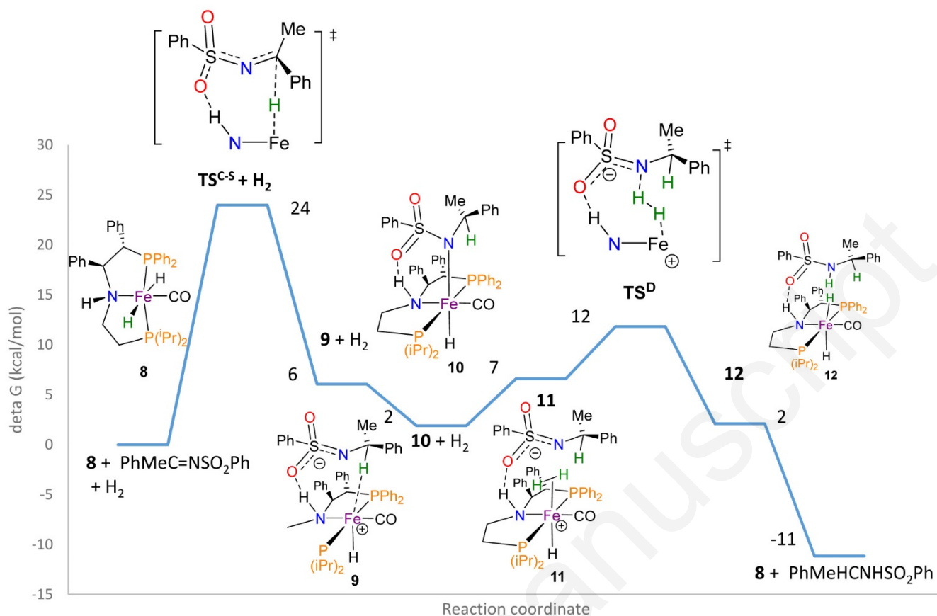
Figure 8. Reaction coordinate diagram (kcal/mol) for a model catalytic cycle for the asymmetric hydrogenation of imine2 catalyzed by the \text{FeH}_2(\text{CO})(\text{P-NH-P}') catalyst 8 where dihydrogen splits into a hydride on iron and a proton on the nitrogen of the outer sphere amide form of the substrate. The \text{H}_2 splitting transition state structure is shown with non essential atoms deleted for clarity. See also Figure S4 for the complete cycle.
