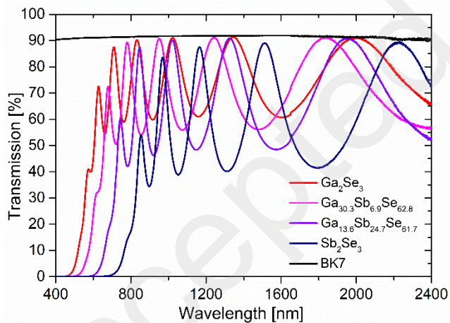
Fig. 1 Transmission spectra of \text{Ga}_2\text{Se}_3 , \text{Ga}_{30.3}\text{Sb}_{6.9}\text{Se}_{62.8} , \text{Ga}_{13.6}\text{Sb}_{24.7}\text{Se}_{61.7} and \text{Sb}_2\text{Se}_3 thin films and BK7 glass substrate.
