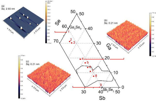
Fig. 2 Ternary Ga-Sb-Se diagram with indicated positions of co-sputtered thin films' composition (red points), targets' composition (black points) and glass-forming region when quenched by fast cooling taken from ref. [8] (black curve). Inserts of AFM scans (5 μm×5 μm) with indicated RMS roughness values Sq of (a) Ga 37.6 Se 62.4 (b) Ga 19.2 Sb 17.5 Se 63.3 and (c) Sb 38.5 Se 61.5 film.
