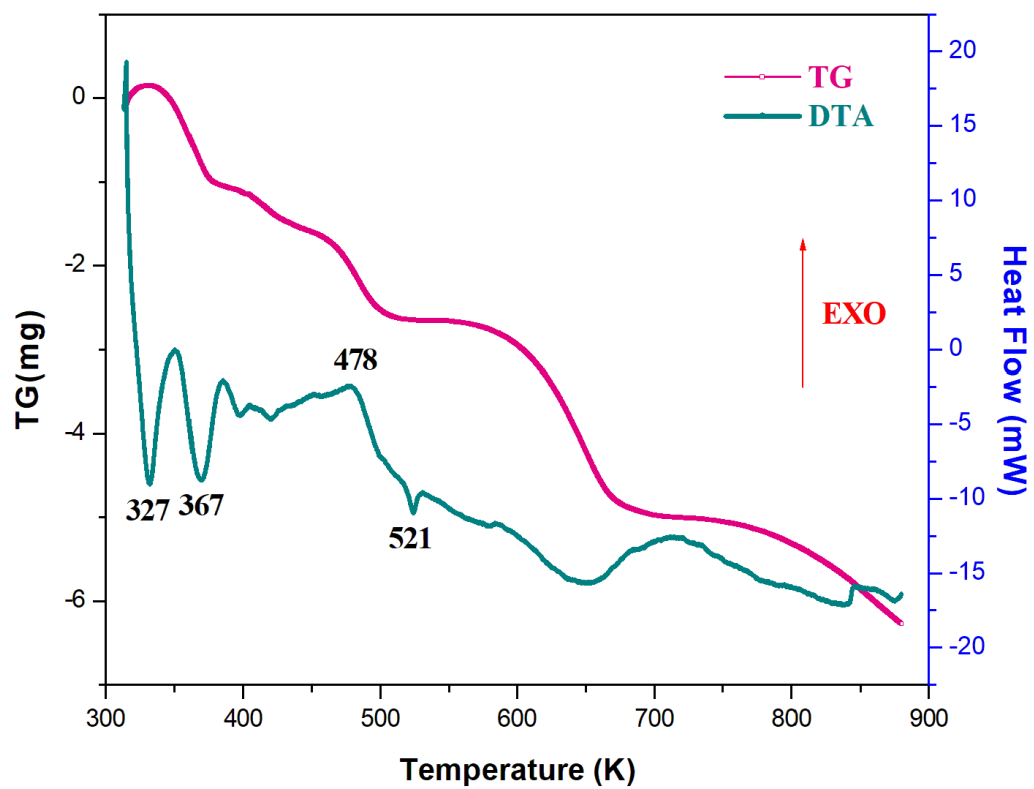
Fig. 10. DTA and TG curves of 2A5PCoCl 4 .
