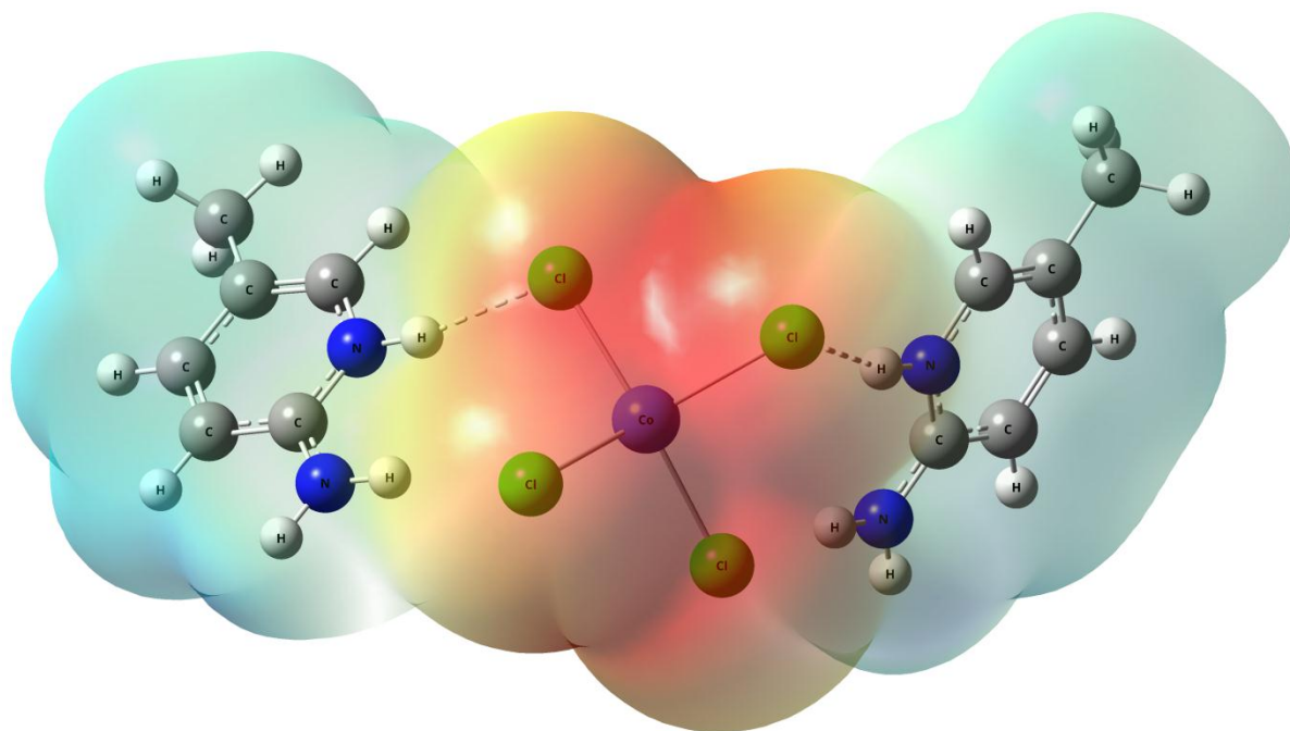
Fig. 9. Molecular Electrostatic Potentials (MEP) surface mapped of 2A5PCoCl 4 .
