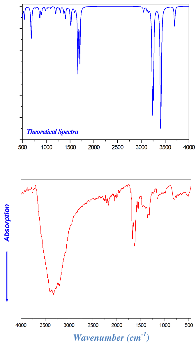
Fig. 8. Theoretical (blue) and experimental (red) IR spectra of 2A5PCoCl 4 .
