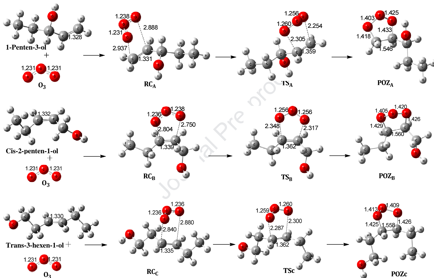
Fig. 5. Optimized geometries of reactants, intermediates, TS, and primary ozonides formed in the reaction of O 3 with A (1-penten-3-ol), B (cis-2-penten-1-ol) and C (trans-3-hexen-1-ol). All are optimized at M06-2x/6-311++G(d,p) level.
