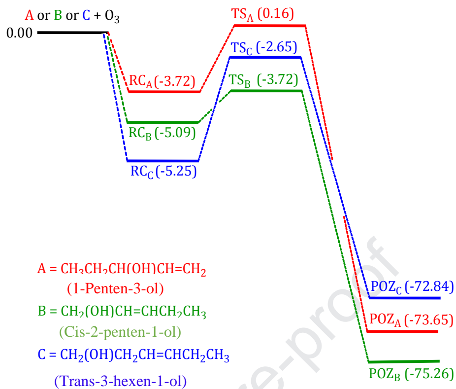
Fig. 6. Energy profile of the reactions of O_3 with the reactants A (red), B (green) and C (blue). Energies are given in kcal/mol.
