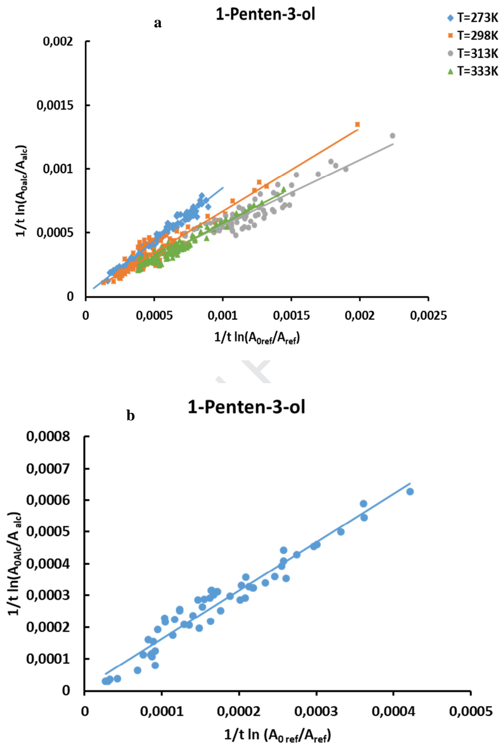
Fig. 1: Plot of 1/t \ln(A_{0alc}/A_{alc}) vs 1/t \ln(A_{0ref}/A_{ref}) for the ozonolysis of 1P3OL at 273, 298, 313 and 333K obtained by FTIR (a) and at T = 298\text{K} by SPME -GC / MS (reference: 1-heptene) (b).
