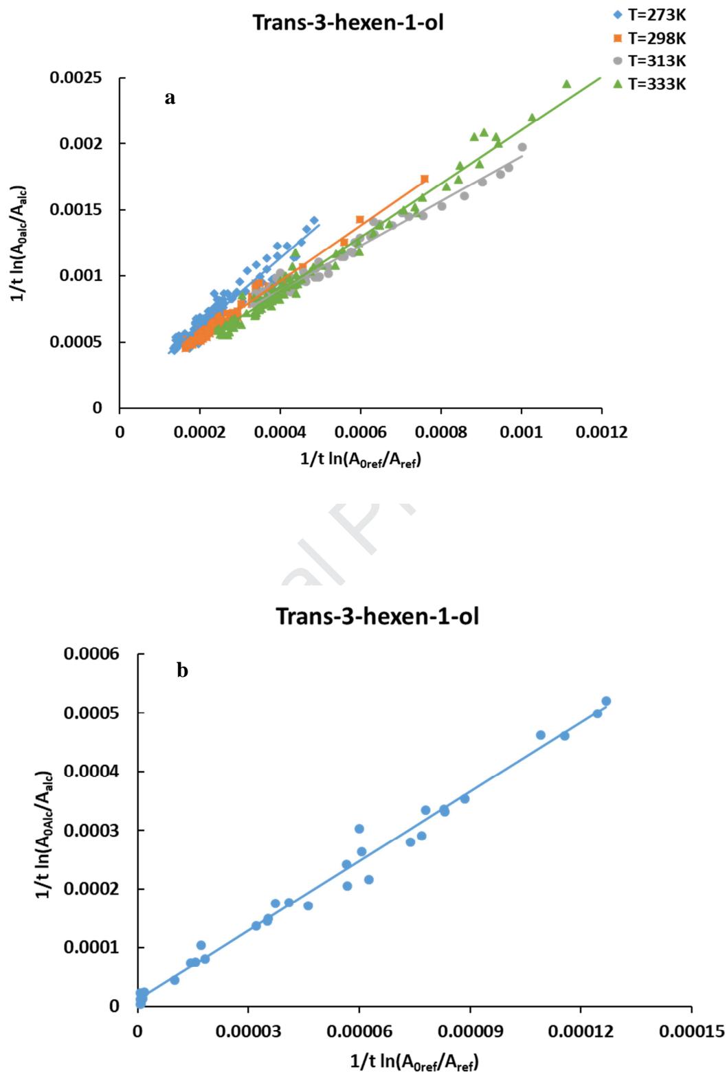
Fig. 3: Plot of 1/t \ln(A_{0alc}/A_{alc}) vs 1/t \ln(A_{0ref}/A_{ref}) for the ozonolysis of t-3H1OL at 273, 298, 313 and 333K obtained by FTIR (a) and at T = 298\text{K} by SPME -GC / MS (reference: 1-penten-3-ol) (b).
