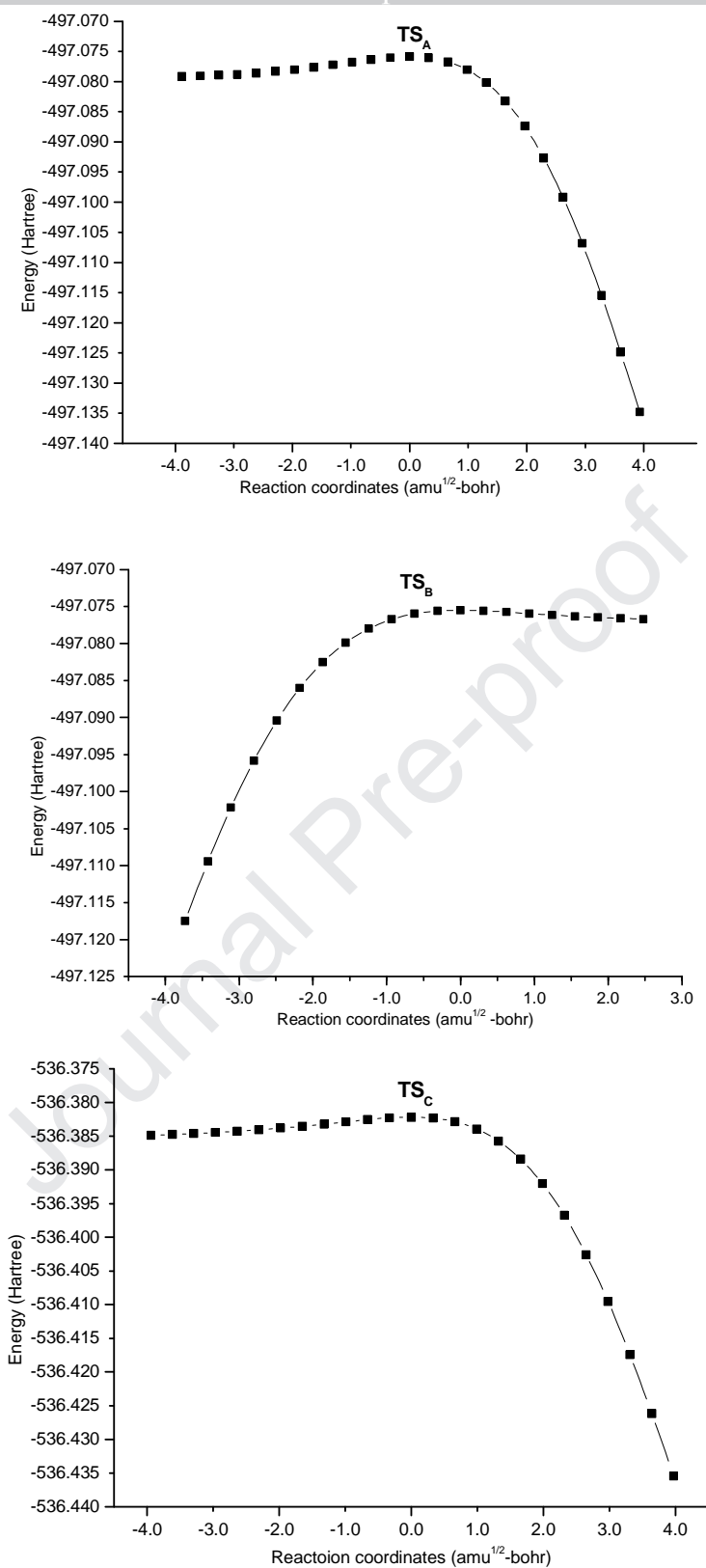
Fig. 7. Intrinsic reaction coordinate (IRC) plots for the TSs of reactions of ozone with A (1-propene-3-ol), B (cis-2-penten-1-ol) and C (trans-3-hexen-1ol).
