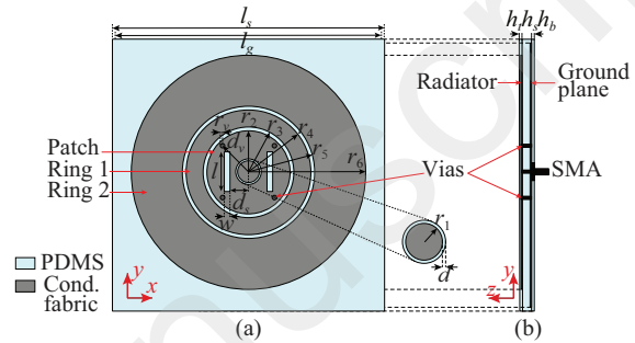
Fig. 1. Proposed antenna geometry: (a) front view, (b) side view. The final dimensions are r_1 = 2.9 , r_2 = 11 , r_3 = 12 , r_4 = 16.5 , r_5 = 17.5 , r_6 = 31 , l_s = 70 , l_g = 68 , l = 10.5 , w = 1.5 , d_s = 4.9 , d_v = 9.7 , r_v = 0.6 , d = 0.5 , h_t = 0.4 , h_s = 3 , and h_b = 0.2 . All dimensions are in millimeters.
