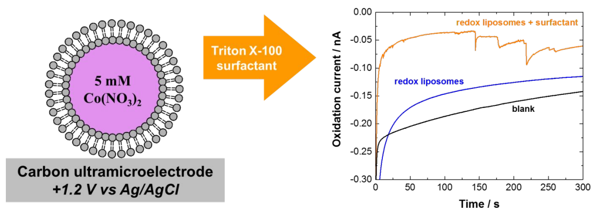
Figure 2. Schematic representation and the i-t curve for collision experiments of redox DMPC liposomes encapsulating 5 mM cobalt(II) nitrate recorded at a 10 \mu m diameter carbon UME polarized at +1.2 V vs. Ag/AgCl in 2 mL of 0.1 M potassium phosphate buffer aqueous solution at pH 7 in the absence (black) and in the presence of 20 \mu L of redox DMPC liposomes aqueous solution with (orange) and without (blue) addition of 0.2 mM Triton X-100 surfactant. Temperature: 20 °C. The UME is not drawn to scale.
