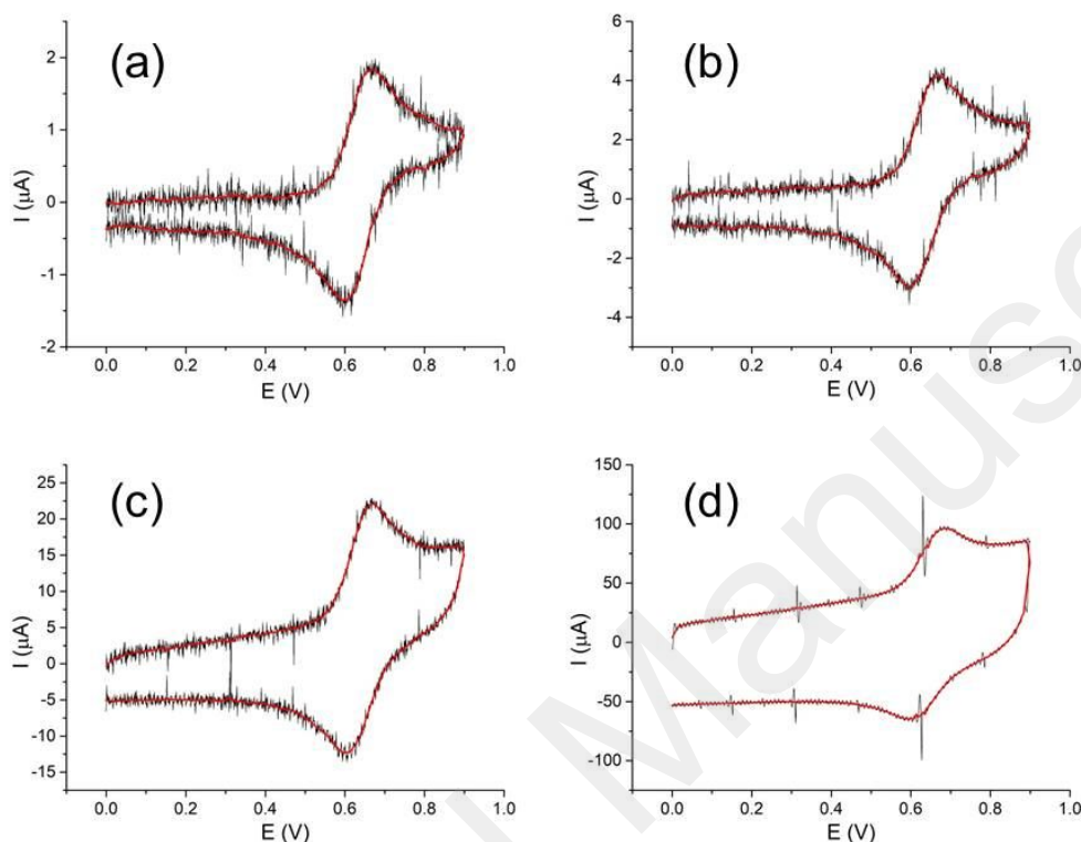
Figure 1. Cyclic voltammograms of the oxidation of a solution of ferrocene in Ethaline ( C^\circ = 2 \times 10^{-3} \text{ mol L}^{-1} ) on a 1-mm diameter glassy carbon electrode at 0.5 (a), 2 (b), 25 (c), 200 (d) V s -1 . Red lines are smooth lines. T = 298 \text{ K} .
