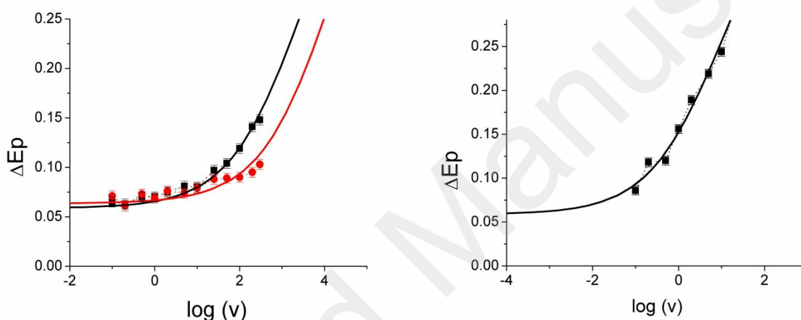
Figure 4. Cyclic voltammetry investigations of the oxidation of a 2 \times 10^{-3} \text{ mol L}^{-1} ferrocyanide solution in Ethaline (left) and in water (+ 0.1 \text{ mol L}^{-1} \text{ KCl} ) (right) on a 1-mm diameter glassy carbon electrode. Variations of \Delta E_p as function of the \log(v) ( v the scan rate in \text{V s}^{-1} ) at different temperatures: in Ethaline T = 308 \text{ K} (black) and 333 \text{ K} (red); in water at 308 \text{ K} (right). Lines are the theoretical variations assuming a Butler-Volmer law and taking \alpha = 0.5 as transfer coefficient.
