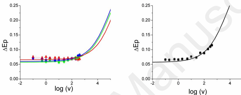
Figure 2. Cyclic voltammetry investigations of the oxidation of a 2 \times 10^{-3} \text{ mol L}^{-1} ferrocene solution in Ethaline (left) and in ACN ( + 0.1 \text{ mol L}^{-1} \text{ nBu}_4\text{NPF}_6 ) (right). Variations of \Delta E_p as function of the \log(v) ( v : scan rate in \text{V s}^{-1} ) at different temperatures: in Ethaline, T=298 (green), 313 (blue), 343\text{K} (red); in acetonitrile at T=298\text{K} . Lines are the theoretical variations assuming a Butler-Volmer law and taking \alpha=0.5 as transfer coefficient (see text).
