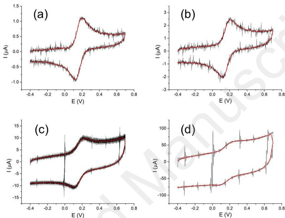
Figure 3. Cyclic voltammograms of the oxidation of a 2 \times 10^{-3} \text{ mol L}^{-1} solution of ferrocyanide in Ethaline on a 1-mm diameter disk glassy carbon at 0.5 (a), 2 (b), 25 (c), 200 (d) \text{V s}^{-1} . Red lines are smooth lines.
