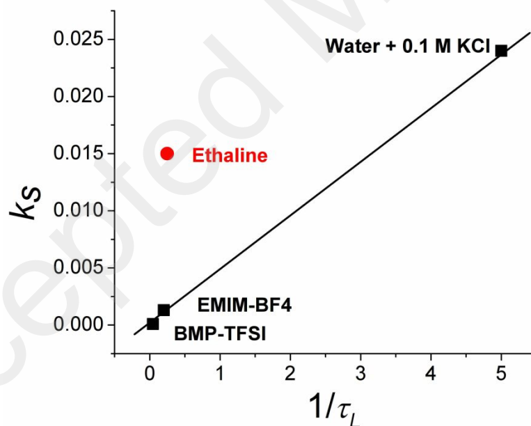
Figure 5. Variations of k_s for the ferrocyanide/ferricyanide couple versus 1/\tau_L , \tau_L , being the longitudinal relaxation time of the solvent. k_s in cm s -1 and \tau_L in ps.
