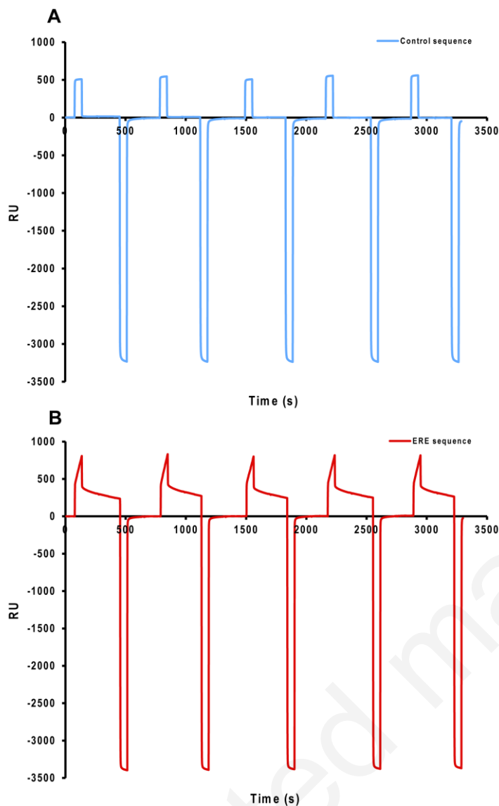
Figure 3: Injection of 40 \mu\text{L} of ER (50 nM) onto (A) a bare SA sensor chip, or (B) a chip coated with 1200 RU of ERE
