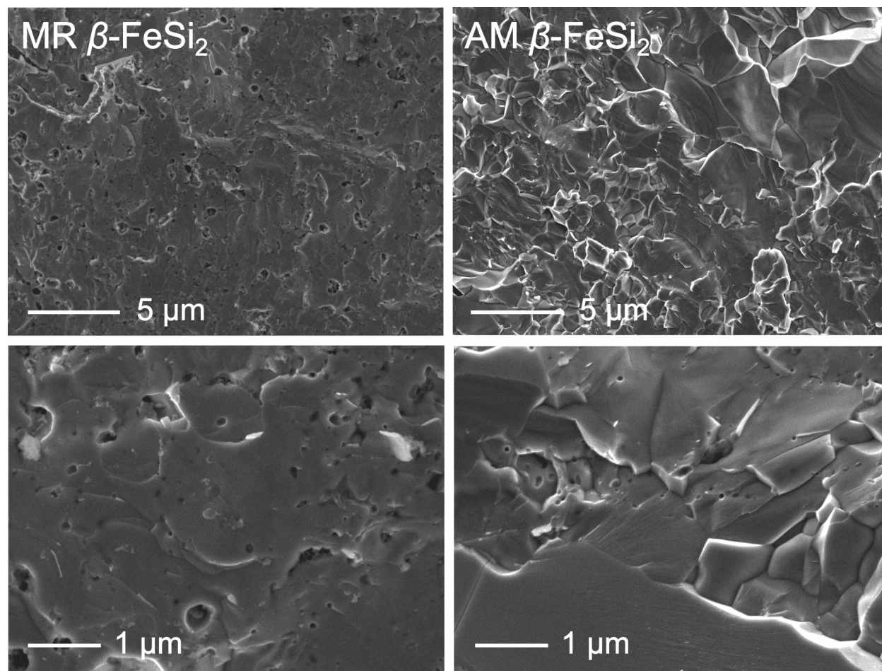
Figure 8: Secondary electron SEM images of broken cross-sections of MR (left side) and AM FeSi 2 (right side) at two different magnifications.
