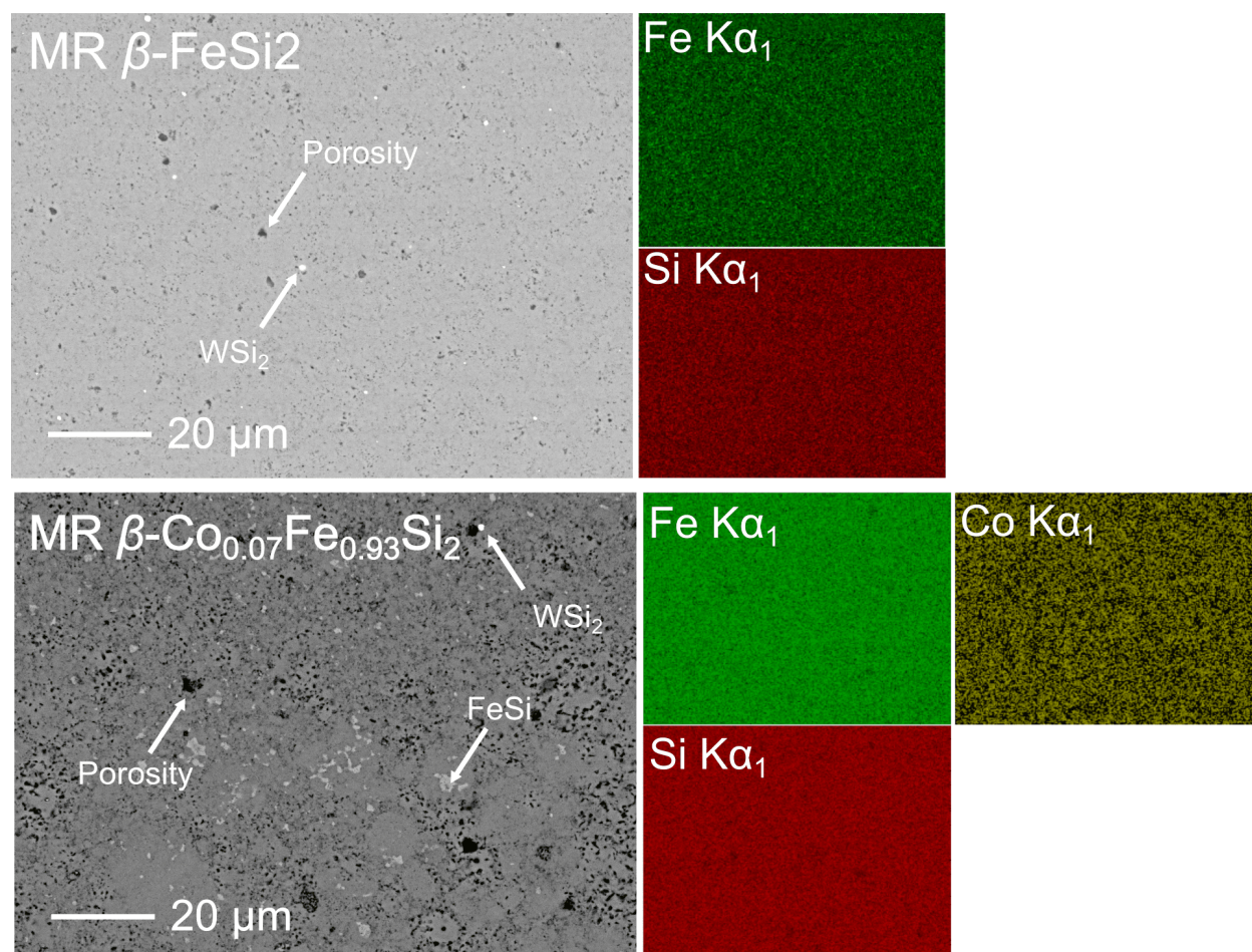
Figure 7: Backscattered electron SEM images and corresponding EDS mappings of the polished surface of undoped MR \beta -FeSi 2 (top) and MR \beta -Co 0.07 Fe 0.93 Si 2 (bottom) densified pellets.
