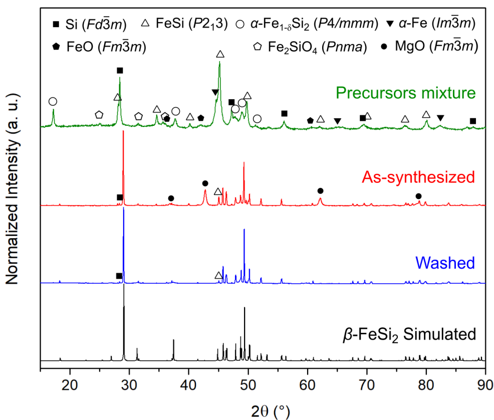
Figure 1: XRD patterns of the precursor mixture (green), as-synthesized (red) and HCl-washed (blue) MR \beta\text{-FeSi}_2 powders, as well as simulated pattern for \beta\text{-FeSi}_2 41 (black). Intensity discrepancies between some peaks in the experimental and theoretical \beta\text{-FeSi}_2 patterns are linked to the presence of (100)[011]/2 stacking faults in the crystals (see text for details).
