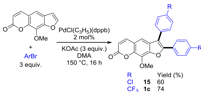
Scheme 5. Pd-catalyzed direct C2,C3-diarylations of Methoxalen using aryl bromides.
