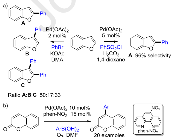
Scheme 3. Regioselectivity of the Pd-catalyzed direct arylations of Methoxalen with a benzenesulfonyl chloride.
