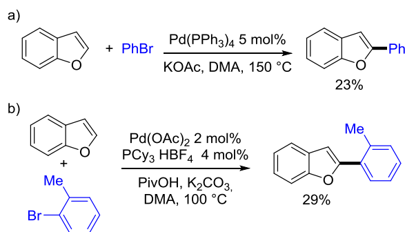
Scheme 1. Pd-catalyzed direct arylations of benzofuran with aryl bromides.
