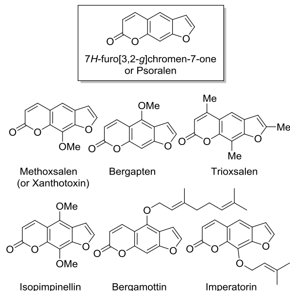
Figure 1. Representative examples of bioactive 7 H -furo[3,2- g ]chromen-7-ones.
