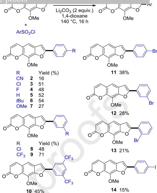
Scheme 4. Pd-catalyzed direct C2-arylations of Methoxalen using benzenesulfonyl chlorides.
