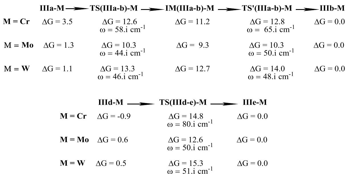
Scheme 5. The stationary points along the \text{IIIa-M} \rightleftharpoons \text{IIIb-M} and \text{IIIId-M} \rightleftharpoons \text{IIIe-M} ( M = \text{Cr, Mo, W} ) IRHR processes and their relative free energies in \text{kcal mol}^{-1} .
