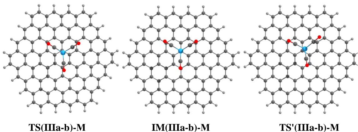
Fig. 9. The transition states and intermediates involved in the \text{IIIa-M} \rightleftharpoons \text{IIIb-M} ( M = \text{Cr, Mo, W} ) \eta^6, \eta^6 -IRHR
