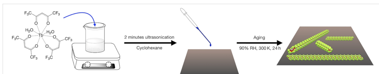
Figure 1: Deposition of [\text{Tb}(\text{hfac})_3 \cdot 2\text{H}_2\text{O}]_n on the mica substrate.
