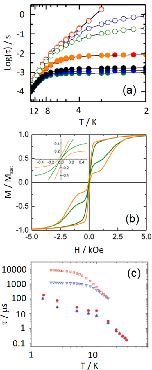
Figure 7. (a) Thermal variation of the magnetic relaxation time \tau of the four isotopologues ^{161}\text{--}^{164}\text{5} (green) (full circles) and diluted samples ^{161}\text{--}^{164}\text{5@Y} (open circles) in a zero magnetic field from 2 to 15 K with blue, orange, green and red colors are attributed to the 161, 162, 163 and 164 isotopes respectively. Full lines are guides to the eye only. (b) Normalized magnetic hysteresis loops at 0.48 K and at a sweep rate of 16 Oe s -1 for ^{162}\text{5@Y} (orange line) and ^{163}\text{5@Y} (green line). The inset is a zoomed view of the origin. (c) Correlation time extracted from muon spectroscopy (full symbols) and relaxation time of magnetization obtained from ac susceptibility (empty symbols) as a function of temperature for ^{161}\text{5} (blue) and ^{164}\text{5} (red). Data are reported on a log-scale. Adapted from refs [96,99].
