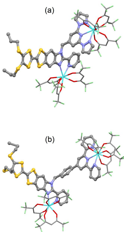
Figure 12. X-ray structures of (a) [Dy 2 (hfac) 6 ( L 5 )]·(CH 2 Cl 2 ) 2 ·C 6 H 14 ( 7 ) and (b) [Dy 2 (hfac) 6 ( L 6 )]·C 6 H 14 ( 8 ). Ligands L 5 and L 6 are represented in ball and sticks and the Dy(hfac) 3 fragment is represented in capped sticks. Color code: carbon: grey, nitrogen: blue, oxygen: red, Sulfur: yellow, fluoride: light green and dysprosium: light blue. Adapted from refs [141,142].
