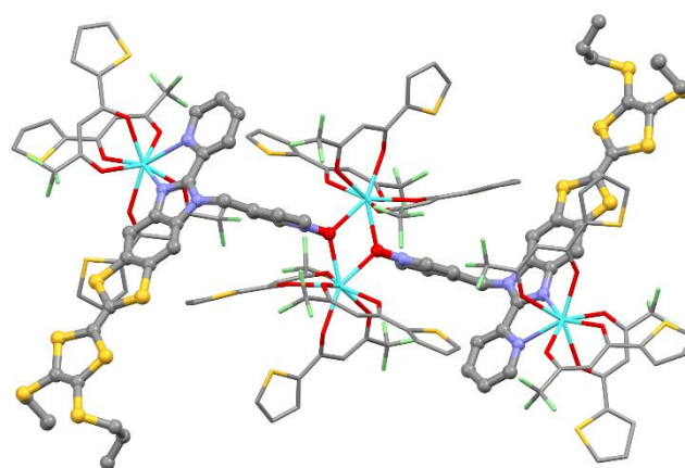
Figure 16. X-ray structure of the tetranuclear [\text{Dy}_4(\text{tta})_{12}(\text{L}^7)_2] \cdot (\text{C}_6\text{H}_{14})_4 complex ( 10 ). Ligand L 7 is represented in ball and sticks and the \text{Dy}(\text{tta})_3 fragment is represented in capped sticks. Color code: carbon: grey, nitrogen: blue, oxygen: red, Sulfur: yellow, fluoride: light green and dysprosium: light blue. Adapted from ref. [158].
