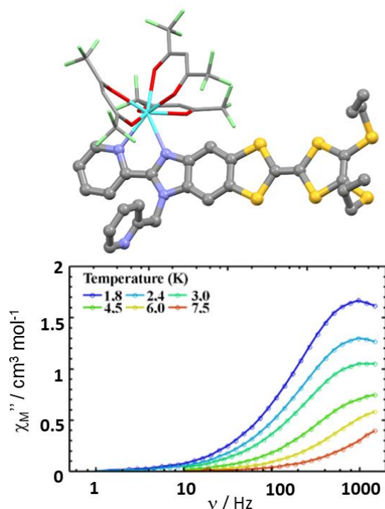
Figure 2. (Top) X-ray structure of [Dy(hfac)_3(L^2)] ( 2 ) and (bottom) the frequency dependence of its out-of-phase signal \chi_M'' measured in solid-state between 1.8 and 7.5 K at H = 0 Oe. Ligand L^2 is represented in ball and sticks and the Dy(hfac)_3 fragment is represented in capped sticks. Color code: carbon: grey, nitrogen: blue, oxygen: red, Sulfur: yellow, fluoride: light green, hydrogen: white and dysprosium: light blue. Adapted from ref [39].
