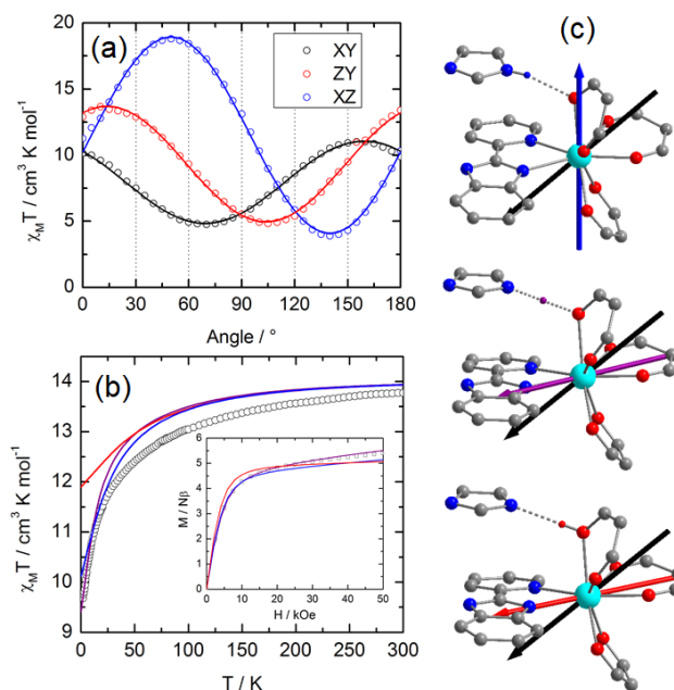
Figure 3. (a) Angular dependence of the \chi_M T product for 1 in the three orthogonal planes (open circles). The full lines represent the best fitted curves. (b) Thermal dependence of the magnetic susceptibility for 1 with the curves calculated on the basis of SA-CASSCF/RASSI-SO data for different positions of the hydrogen atom involved in the hydrogen bond ( H_N , blue line; H_m , purple line and H_O , red line) (c) Orientation of the experimental ground-state anisotropy axes (black arrow) and calculated ground-state anisotropy axis in function of the positions of the hydrogen atom ( H_N , blue arrow; H_m , purple arrow and H_O , red arrow). Color code: carbon: grey, nitrogen: blue, oxygen: red and dysprosium: light blue. Adapted from ref [40].
