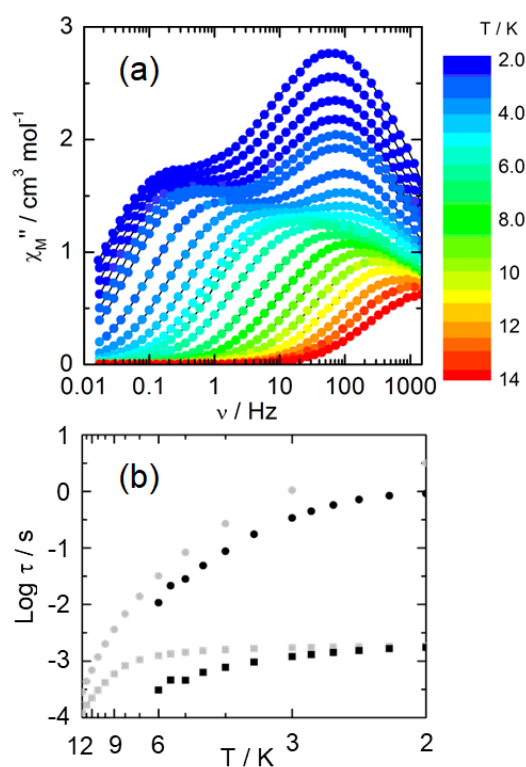
Figure 17. (a) Temperature and frequency dependence of the out-of-phase component of the ac susceptibility measured in zero applied magnetic field for 10 . (b) Temperature dependence of the slow (black disks) and fast (black squares) regimes of 10 measured in zero applied magnetic field. The thermal variation of the logarithm of the relaxation times for isolated 9 (grey disks) and 5 (grey squares) are represented for comparison. Adapted from ref. [158].
