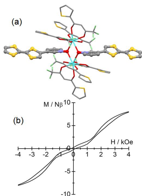
Figure 15. (a) X-ray structure of the dinuclear complex [\text{Dy}(\text{tta})_3(\text{L})]_2 \cdot 0.5\text{CH}_2\text{Cl}_2 ( 9 ). Color code: carbon: grey, nitrogen: blue, oxygen: red, Sulfur: yellow, fluoride: light green and dysprosium: light blue. (b) Magnetic hysteresis loop at 0.48 K and a sweep rate of 16 \text{ Oe s}^{-1} for 9 . Ligand L is represented in ball and sticks and the \text{Dy}(\text{tta})_3 fragment is represented in capped sticks. Adapted from ref. [149].
