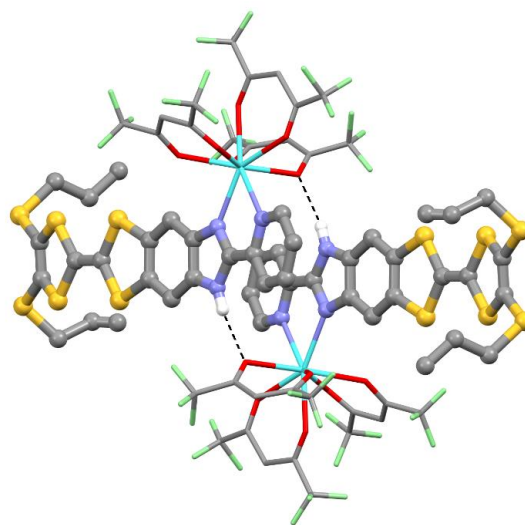
Figure 1. Representation of two neighboring complexes of [Dy(hfac)_3(L^1)] ( 1 ) forming a dimer through hydrogen bonds. Ligand L^1 is represented in ball and sticks while the Dy(hfac)_3 fragment is represented in capped sticks. Color code: carbon: grey, nitrogen: blue, oxygen: red, Sulfur: yellow, fluoride: light green, hydrogen: white and dysprosium: light blue. Adapted from ref [39].
