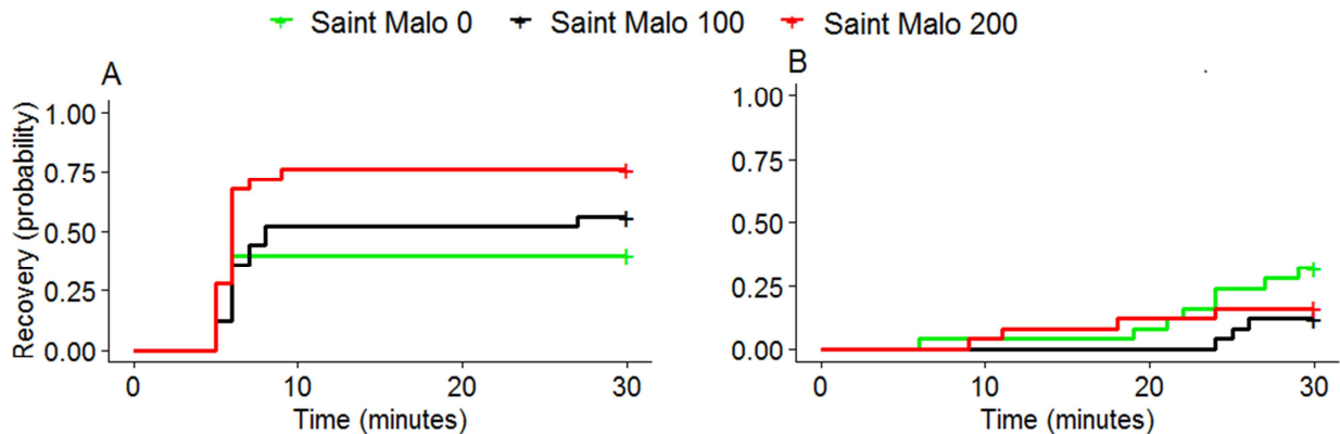
Figure 3 Recovery curves of adult Merizodus soledadinus from three different populations sampled along an altitudinal gradient at the Kerguelen Islands after the insects were exposed to A) -7 °C for 15 minutes (The recovery curves were not significantly different, P = 0.056 ). B) 37 °C for 15 minutes (The recovery curves were not significantly different, P = 0.17 ). Recovery curves were estimated using the Kaplan Meier method; vertical tick-marks represent insects that did not recover at the end of the 30 min recovery period (“right censored data”).
