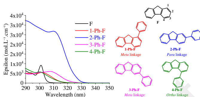
Figure 3. Absorption spectra in cyclohexane (Left) and molecular structures (Right) of 1-Ph-F , 2-Ph-F , 3-Ph-F and 4-Ph-F and F .
