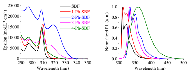
Figure 2. 1-Ph-SBF , 2-Ph-SBF , 3-Ph-SBF and 4-Ph-SBF . Top. ORTEP drawing (ellipsoid probability at 50 % level) from X-Ray crystallography, Bottom. Absorption (Left) and emission (Right) spectra in cyclohexane ( SBF is added for comparison purpose)
