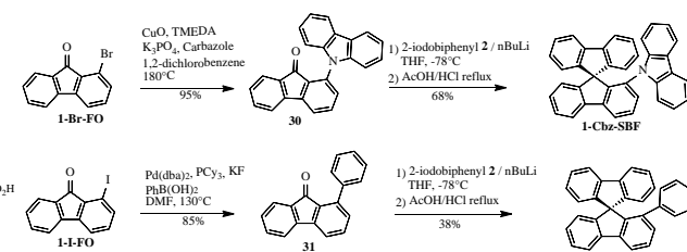
Scheme 7. Synthesis of 1-substituted SBFs 1-Cbz-SBF and 1-Ph-SBF
