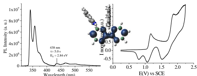
Figure 14: 1-Cbz-SBF . Left. Emission spectrum at 77 K (2-Me-THF, \lambda_{exc} = 300 nm), inset. SDD (isovalence = 0.004). Right. CV (100 \text{mV s}^{-1} , \text{CH}_2\text{Cl}_2/\text{Bu}_4\text{NPF}_6 , 0.2 M).
