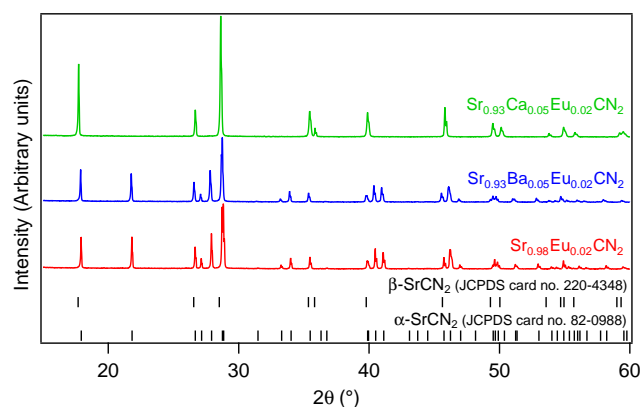
Figure 3: The X-ray diffraction diagrams of Eu 2+ doped SrCN 2 samples (Sr 0.98 Eu 0.02 CN 2 , Sr 0.93 Ba 0.05 Eu 0.02 CN 2 and Sr 0.93 Ca 0.05 Eu 0.02 CN 2 , red, blue and green curves, respectively).
