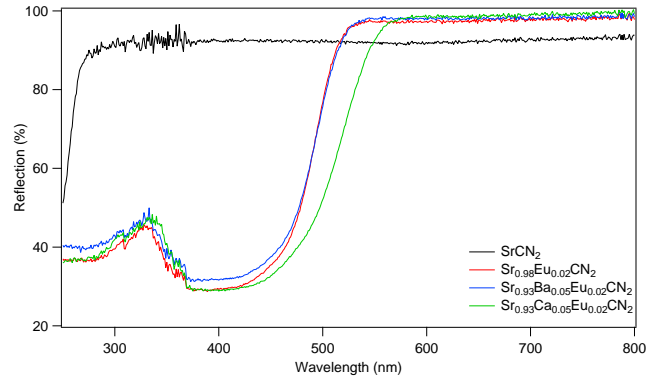
Figure 4: Diffuse Reflectance spectra of undoped ( \text{SrCN}_2 , black curve) and \text{Eu}^{2+} doped \text{SrCN}_2 samples ( \text{Sr}_{0.98}\text{Eu}_{0.02}\text{CN}_2 , \text{Sr}_{0.93}\text{Ba}_{0.05}\text{Eu}_{0.02}\text{CN}_2 and \text{Sr}_{0.93}\text{Ca}_{0.05}\text{Eu}_{0.02}\text{CN}_2 , red, blue and green curves, respectively).
