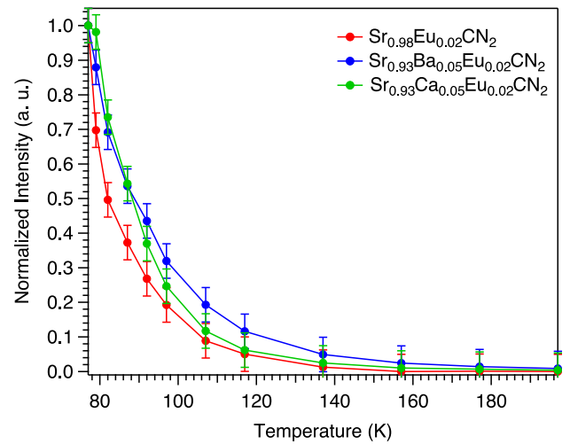
Figure 6: Normalized emission intensity (integrated area) vs temperature (77 - 197 K) for Sr 0.98 Eu 0.02 CN 2 (red points), Sr 0.93 Ba 0.05 Eu 0.02 CN 2 (blue points), Sr 0.93 Ca 0.05 Eu 0.02 CN 2 (green points). Uncertainty bar = \pm 0.05 .
