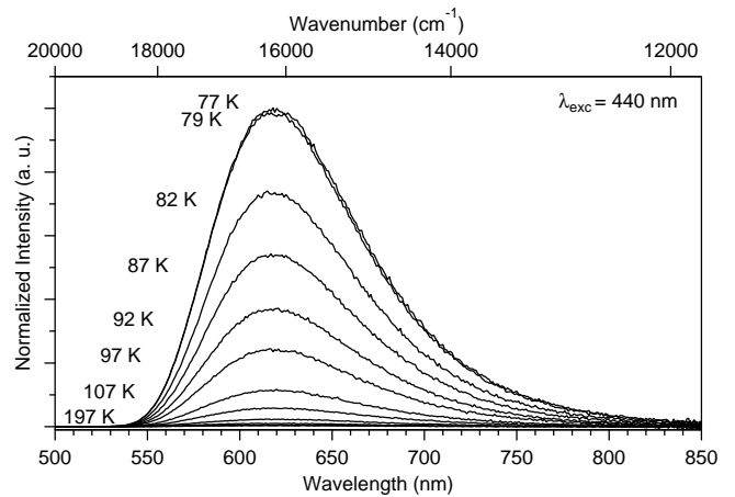
Figure S7: Emission ( \lambda_{\text{ex}} = 440 \text{ nm} ) spectra of \text{Sr}_{0.93}\text{Ca}_{0.05}\text{Eu}_{0.02}\text{CN}_2 at variable temperature (77 - 197 K).
