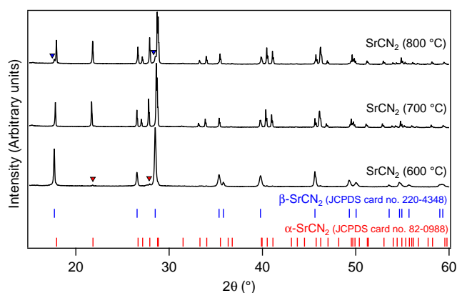
Figure 2: The X-ray diffraction diagrams of SrCN 2 samples synthesized at different temperatures (from 600 to 800 °C). Blue triangles indicate extra-peaks corresponding to \beta -SrCN 2 phase while red triangles indicate extra-peaks corresponding to \alpha -SrCN 2 .
