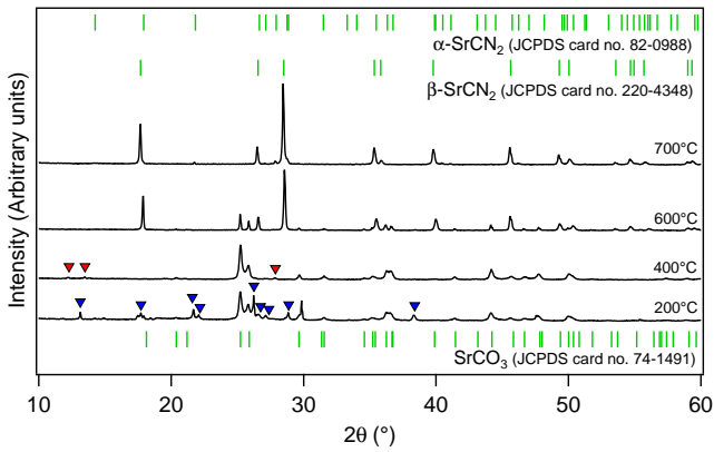
Figure S2: Powder XRD patterns of the products obtained from mixtures of \text{H}_2\text{CN}_2 and \text{SrCO}_3 at various temperatures. Blue triangles indicate extra-peaks corresponding to melamine phase while red triangles indicate extra-peaks corresponding to melem phase.
