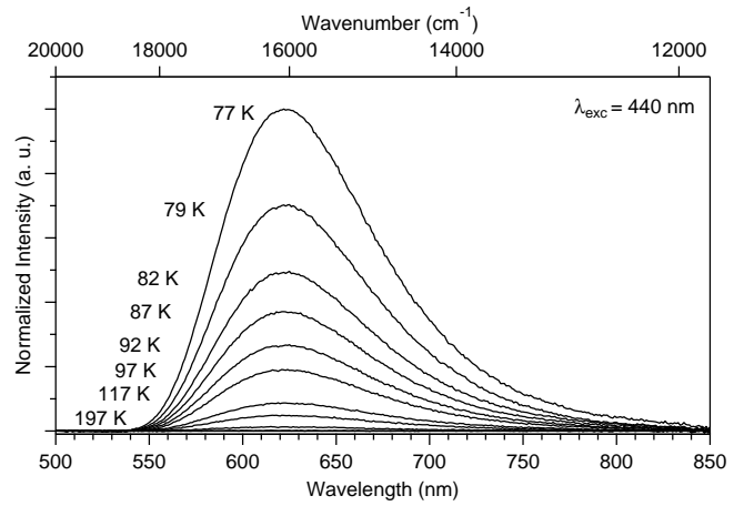
Figure S5: Emission ( \lambda_{\text{ex}} = 440 \text{ nm} ) spectra of \text{Sr}_{0.98}\text{Ba}_{0.05}\text{Eu}_{0.02}\text{CN}_2 at variable temperature (77 - 197 K).
