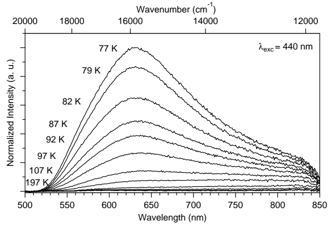
Figure S6: Emission ( \lambda_{\text{ex}} = 440 \text{ nm} ) spectra of \text{Sr}_{0.93}\text{Ba}_{0.05}\text{Eu}_{0.02}\text{CN}_2 at variable temperature (77 - 197 K).
