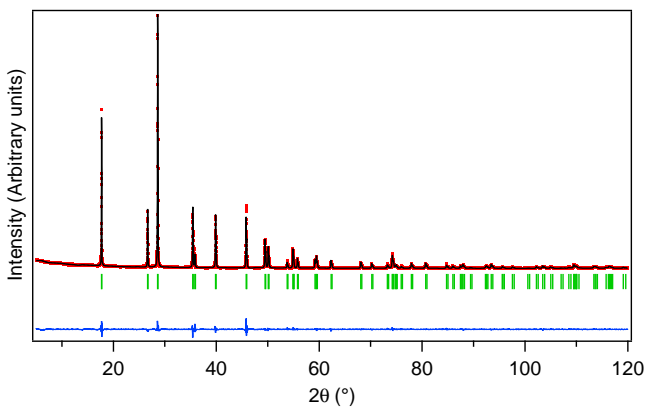
Figure S4: Final Rietveld refinement pattern for \text{Sr}_{0.93}\text{Ca}_{0.05}\text{Eu}_{0.02}\text{CN}_2 : observed (red dotted line), calculated (black full line) and difference (blue line) X-ray powder diffraction profiles from the pattern matching plot obtained with Fullprof. The vertical markers correspond to the position of the Bragg reflections.
