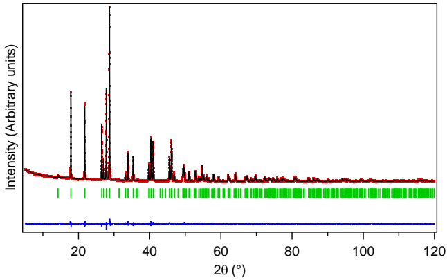
Figure S3: Final Rietveld refinement pattern for \text{Sr}_{0.93}\text{Ba}_{0.05}\text{Eu}_{0.02}\text{CN}_2 : observed (red dotted line), calculated (black full line) and difference (blue line) X-ray powder diffraction profiles from the pattern matching plot obtained with Fullprof. The vertical markers correspond to the position of the Bragg reflections.
