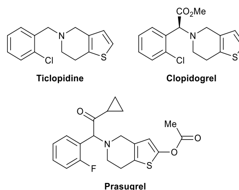
Figure 1. Structures of Ticlopidine, Clopidogrel and Prasugrel.
