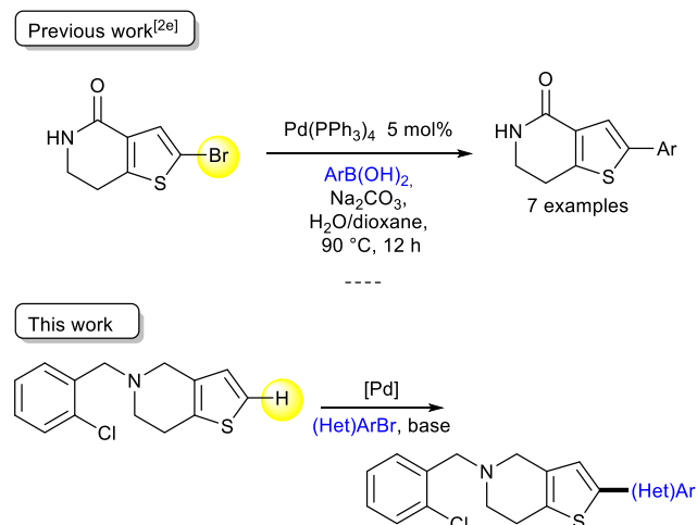
Scheme 1. Access to arylated thienopyridine derivatives.
