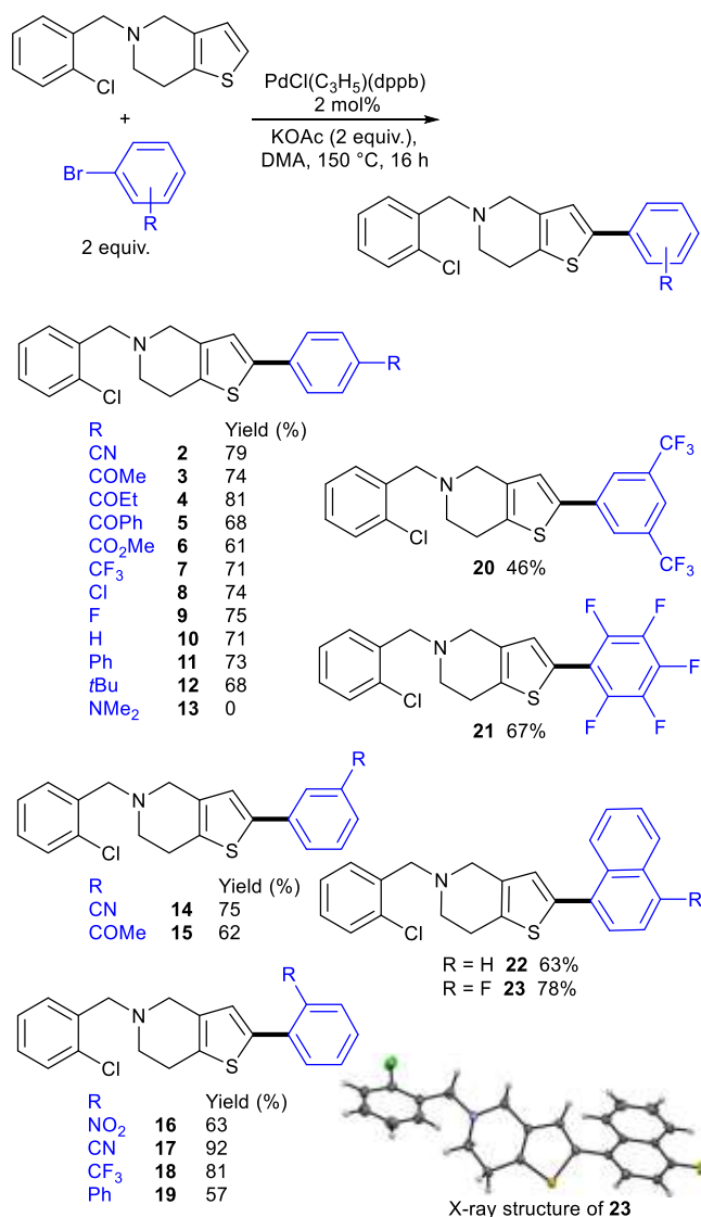
Scheme 2. Synthesis of arylated Ticlopidine derivatives.
