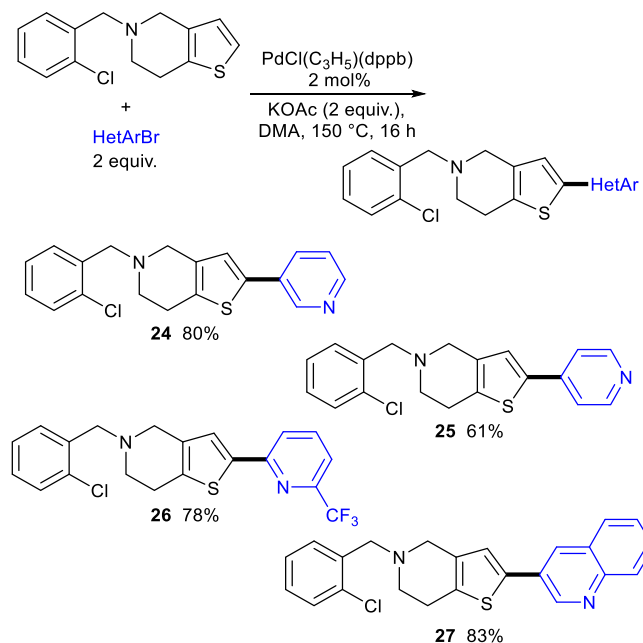
Scheme 3. Synthesis of heteroarylated Ticlopidine derivatives.
