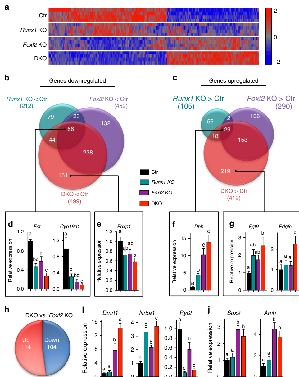
Fig. 7 Transcriptomic analysis of XX Runx1 / Foxl2 single and double KO ovaries. a Heat map for the 918 genes differentially expressed in XX Runx1 / Foxl2 double knockout (DKO) vs. XX control (Ctr) gonads at birth. The heat map shows the expression of these 918 genes in XX control, Runx1 KO, Foxl2 KO, and Runx1 / Foxl2 DKO gonads (microarray; n = 4 /genotype; one-way ANOVA; fold change > 1.5 , p < 0.05 ). Controls correspond to XX wild-type littermates. b, c Venn diagram comparing the genes downregulated ( b ) or upregulated ( c ) in XX Runx1 KO (green circle), XX Foxl2 KO (purple circle), and XX Runx1 / Foxl2 DKO (red circle) gonads at birth. d–g Validation by quantitative PCR of genes identified in the Venn diagrams as significantly downregulated in all three KO ( d ), or only in Runx1 / Foxl2 DKO ( e ), or significantly upregulated in all in all three KO ( f ) or only in Runx1 / Foxl2 DKO ( g ). h, i Identification of the genes differentially expressed in XX Runx1 / Foxl2 DKO vs. XX Foxl2 KO gonads and validation of candidate genes by quantitative PCR. j Expression of Sox9 and Amh is not changed in XX Runx1 / Foxl2 DKO compared with XX Foxl2 KO gonads. For all the qPCR data, values are presented as mean \pm SEM ( n = 5 /genotype). One-way ANOVA, p < 0.05 . Bars with different letters ( a, b, c ) are significantly different. Source data are provided as a Source Data file
