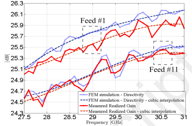
Fig 11. Measured realized gain (red curve) and simulated directivity (blue curve) of the PPW beamformer for feeds #1 ( \theta_1 = 1.5^\circ ) and #11 ( \theta_1 = 31.5^\circ ) over the entire Ka-downlink frequency band ( [27.5-31] GHz).
