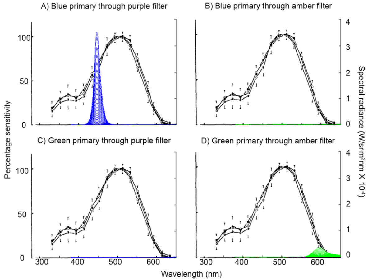
Fig. S1: Spectral transmittance measurements for the anaglyph 3D glasses. Spectral radiance of light across different wavelengths as transmitted through the filters (y-axis on the right) compared to the mantis spectral sensitivity curve reproduced from Rossel (1979) (y-axis on the left). Different individual curves show spectral radiance measured at increasing digital driving levels. Filters used were LEE filters: Filter 797 Purple and Filter 135 Deep Golden Amber. A) Light from the blue primary transmitted through the purple filter. B) Light from the blue primary transmitted through the amber filter. C) Light from the green primary transmitted through the purple filter. D) Light from the green primary transmitted through the amber filter.
