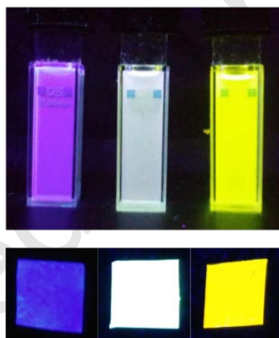
Figure 13. Top: Changes in the color of a solution of 52 ( c = 1.25 \times 10^{-5} M in CH 2 Cl 2 , left) after addition of 45 equivalents (middle) and in 10^{-2} M CSA (right). Bottom: Changes in the color of filter paper samples after immersion in a CH 2 Cl 2 solution of polystyrene doped with 52 (1 wt%) in the absence (left) and presence of 0.1 equivalents (middle) and 80 equivalents (right) of camphorsulfonic acid. Photographs were taken upon irradiation with a hand-held UV-lamp ( \lambda_{\text{exc}} = 366 nm).
