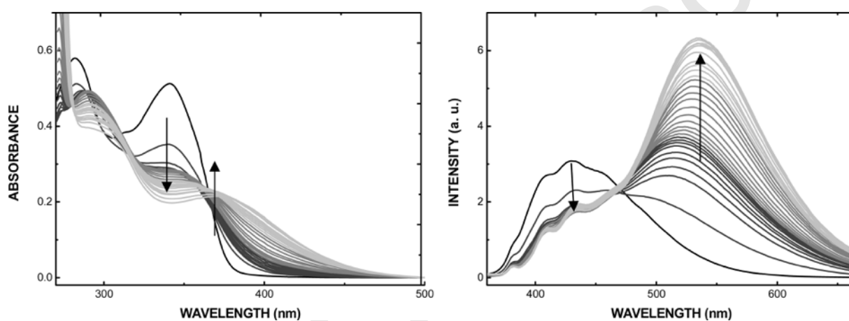
Figure 4. Changes in the absorption (left) and emission (right) spectra of 10 ( 2.0 \times 10^{-5} M in THF) upon addition of p -TSA ( 7.5 \times 10^{-5} M to a large excess). Reproduced with permission from reference [23] (copyright 2011 American Chemical Society).
