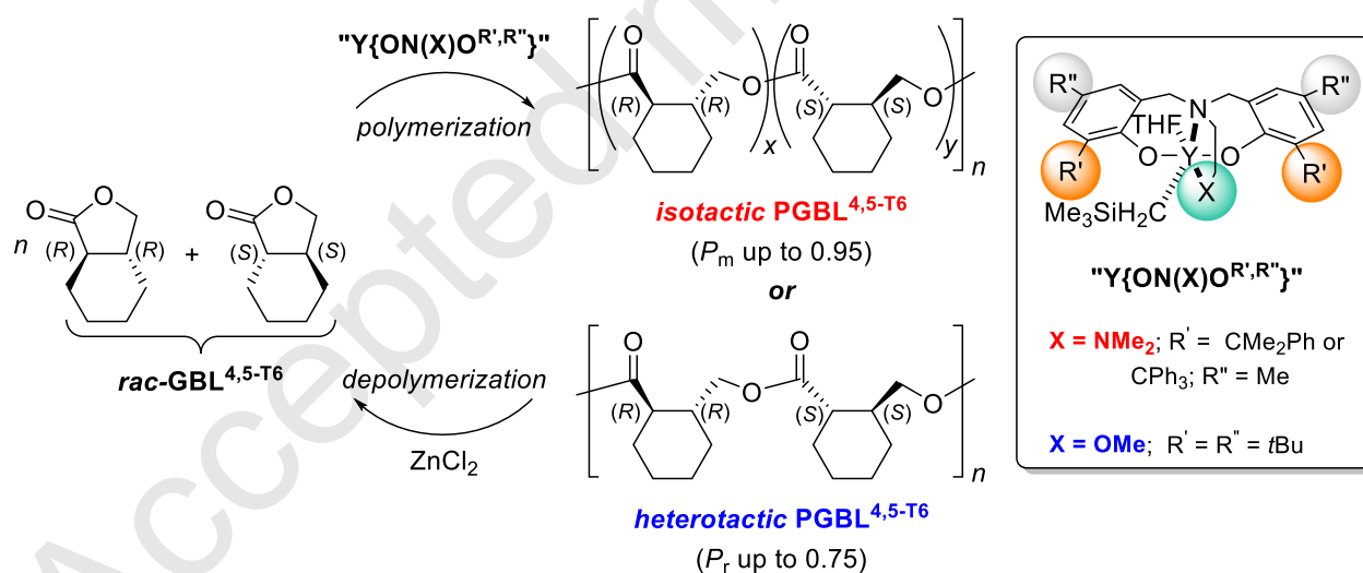
Scheme 3. Access to isotactic or heterotactic \text{PGBL}^{4,5\text{-T6}} with full recyclability from the ROP of racemic trans -cyclohexyl-ring-fused \gamma -butyrolactone ( \text{rac-GBL}^{4,5\text{-T6}} ) with achiral yttrium complexes. [18]
