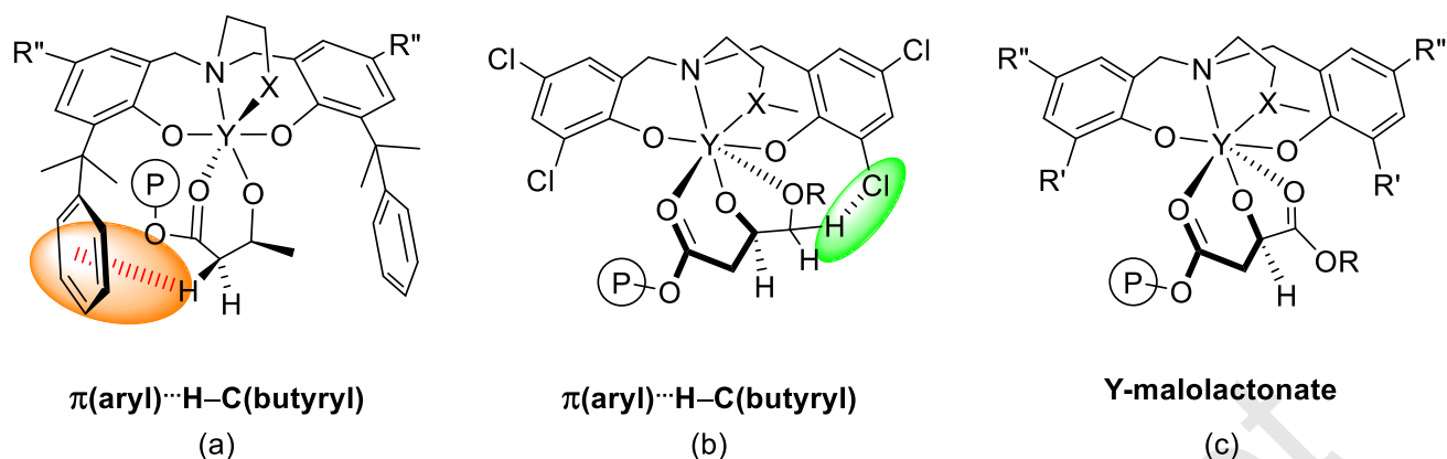
Chart 2. Illustration of putative “non-covalent interactions” (NCIs) at work in stereoselective ROP of rac -BL Me (a), rac -BPL OR (b), and of the multi-coordinated species in ROP of rac -MLA R (c) with yttrium{ON(X)O R',R'' } catalysts. [6b,10]
