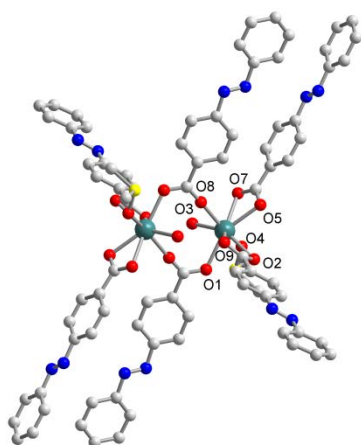
Figure 1. Representation of the dimer found in DyAZO (Dy, teal; O, red; C, grey; N, blue; S, yellow). Hydrogen atoms and free solvent molecules omitted for clarity.
