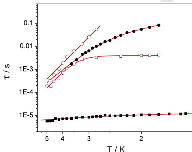
Figure 6. Relaxation times as a function of the temperature for DyAZO (filled symbols) and YDyAZO (empty symbols), measured with H_{dc} = 0 Oe (squares) and H_{dc} = 1200 Oe (circles). Red lines are the best fits discussed in the text.
