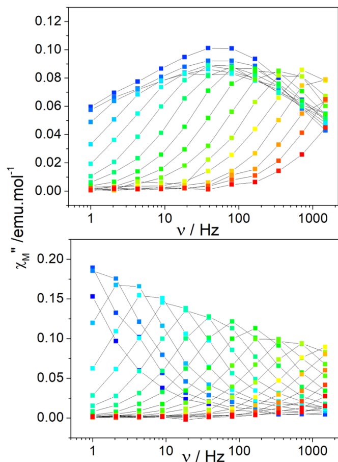
Figure 5. Frequency dependence of the out-of-phase component of the magnetization measured on YDyAZO with H_{dc} = 0 Oe, 1.6 K - 5 K (top) and H_{dc} = 1200 Oe, 1.6 K - 5 K (bottom).
