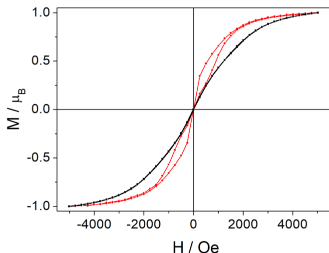
Figure 7. Hysteresis curves measured for DyAZO (black) and YDyAZO (red) at 0.5 K with a sweep rate of 15.5 \text{ Oe}\cdot\text{s}^{-1} .
