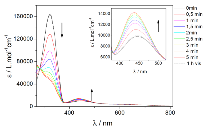
Figure 8. UV/Vis absorption spectra of a 1,4-dioxane solution ( 1 \times 10^{-5} \text{ mol}\cdot\text{L}^{-1} ) of DyAZO upon irradiation under UV light ( \lambda_{\text{exc}} = 365 \text{ nm} , irradiance E_e = 2.40 \text{ mW}\cdot\text{cm}^{-2} ) and after 1 hour at ambient visible light.
