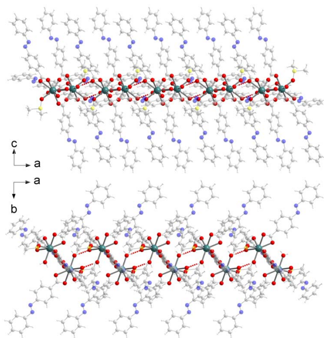
Figure 2. Representation of the supramolecular chain in DyAZO along the b (top) and c axis (bottom). Intermolecular H bonds as red dashed bonds. Free solvent molecules omitted for clarity.
