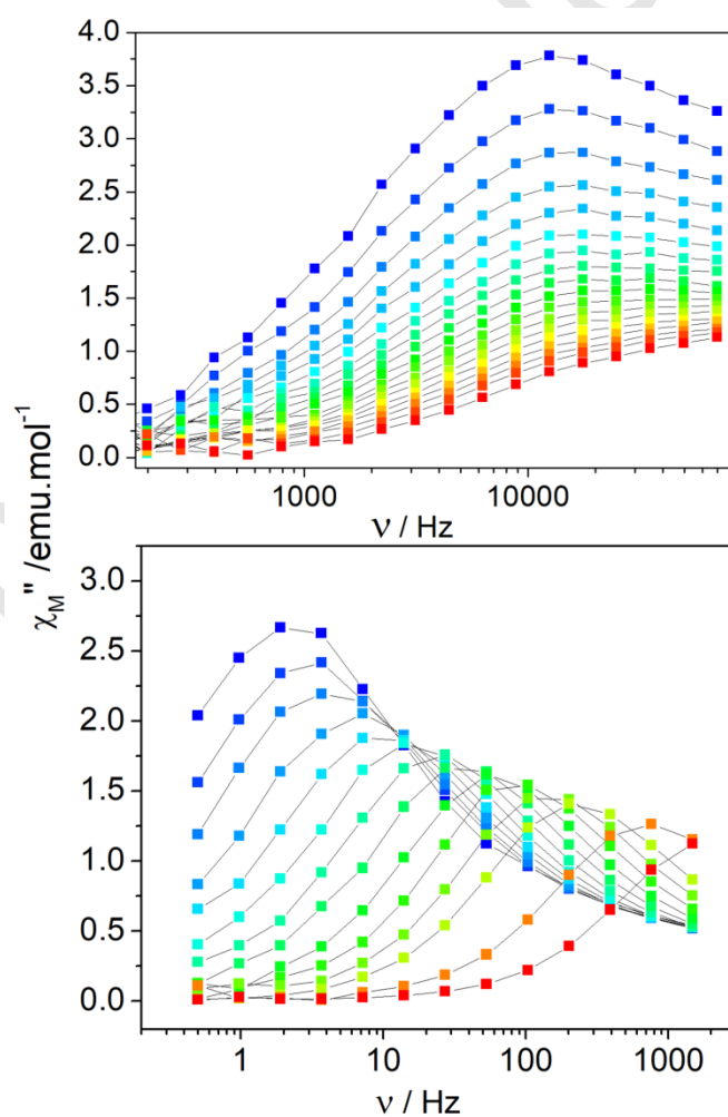
Figure 4. Frequency dependence of the out-of-phase component of the magnetization measured on DyAZO with H_{dc} = 0 Oe, 1.6 K-7.6 K (top) and H_{dc} = 1200 Oe, 1.8 K – 5 K (bottom).
