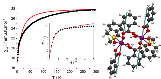
Figure 3. (left) Experimental (black dot) and calculated (red curve) temperature dependence of the \chi_M T product for DyAZO and field dependence of the magnetization at 2 K in inset. (right) Orientation of the calculated easy magnetization axes for the ground state of the Dy^{3+} centers (Dy, teal; O, red; C, grey; N, blue; S, yellow).
