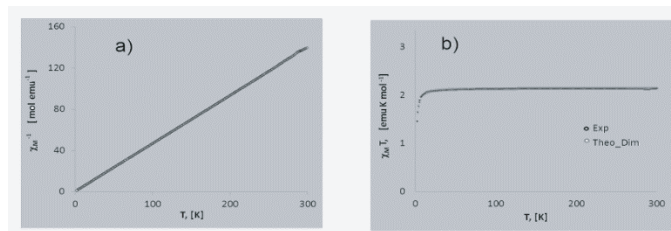
Fig. 4. Magnetic behavior of complex (1) a) Temperature dependence of \chi_M^{-1} b) Temperature dependence of \chi_M T in the range from 2 to 300 K.
