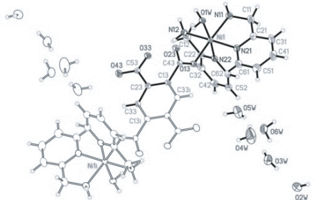
Fig. 1. The dinuclear unit in (1). (Displacement factors at a 50% level).
