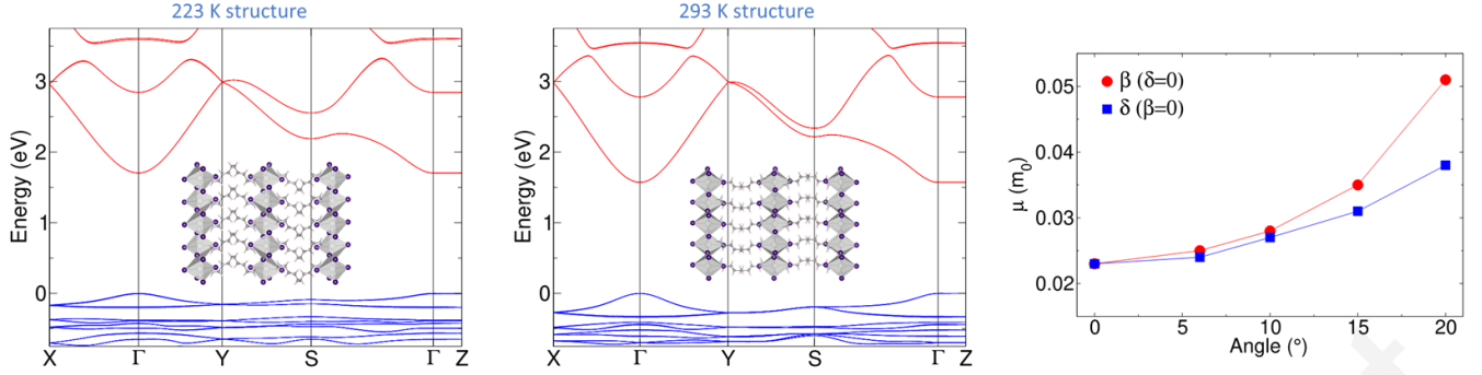
Figure 4: Band structure corresponding to LT (a) and HT (b) phases of (C_4H_9NH_3)_2PbI_4 together with schematic crystal structure for high and low temperature phase). (c) Dependence of reduced exciton mass versus \beta and \delta angles.
