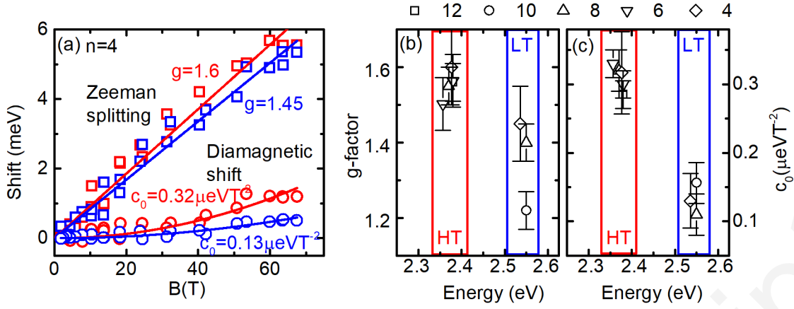
Figure 3: (a) Comparison of Zeeman (open squares) and diamagnetic shifts (open circles) for the LT (blue) and HT (red) phases for (\text{C}_4\text{H}_9\text{NH}_3)_2\text{PbI}_4 . (b) Measured g-factors and (c) diamagnetic coefficients as a function of transition energy. Symbols correspond to different number of carbon atoms in organic spacer.
