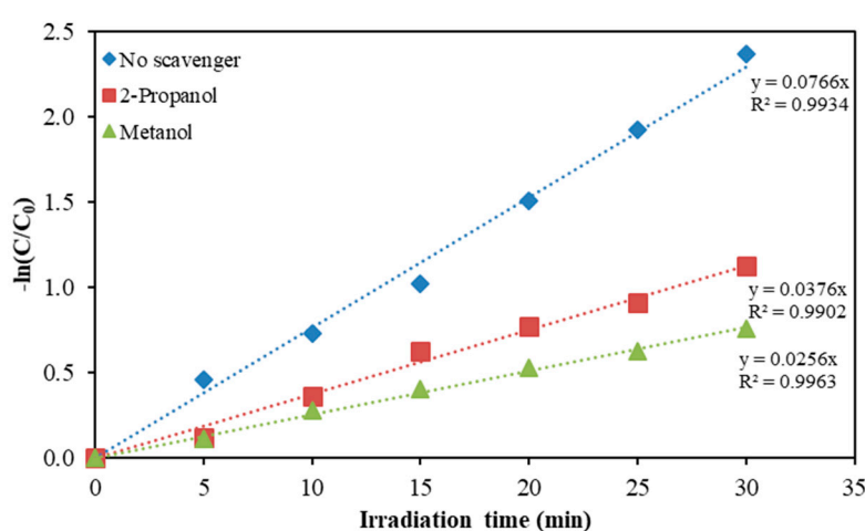
Figure 6. Photocatalytic degradation kinetics of the target molecule in the absence and presence of the selected chemical scavengers (0.1 M). Initial clofibrac acid concentration of 1.5 mg/L, 1 g/L catalyst load, 9.52 mW/cm 2 , room temperature.
