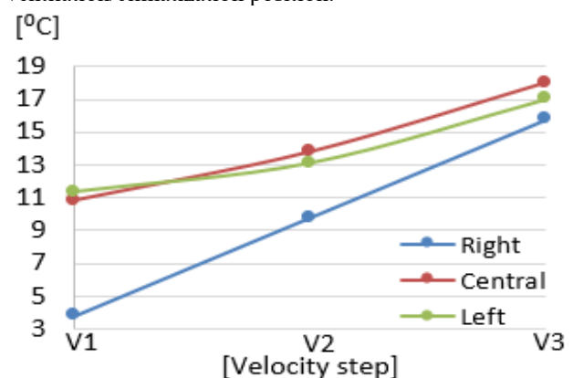
Fig. 6. Inlet jet air temperature
