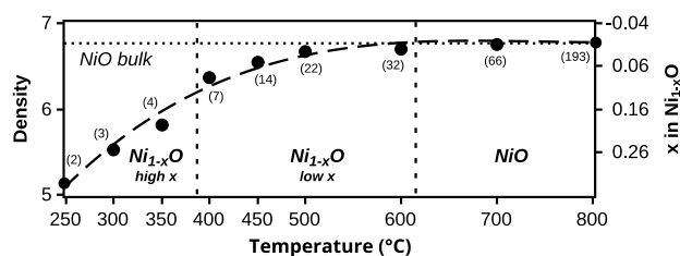
Figure 2. Evolution of the density and the Ni off-stoichiometry of NiO-T samples versus their synthesis temperature. The dashed line has to be regarded as a guide to the eyes. Calculated crystallite sizes (in nanometers) are indicated within brackets.
