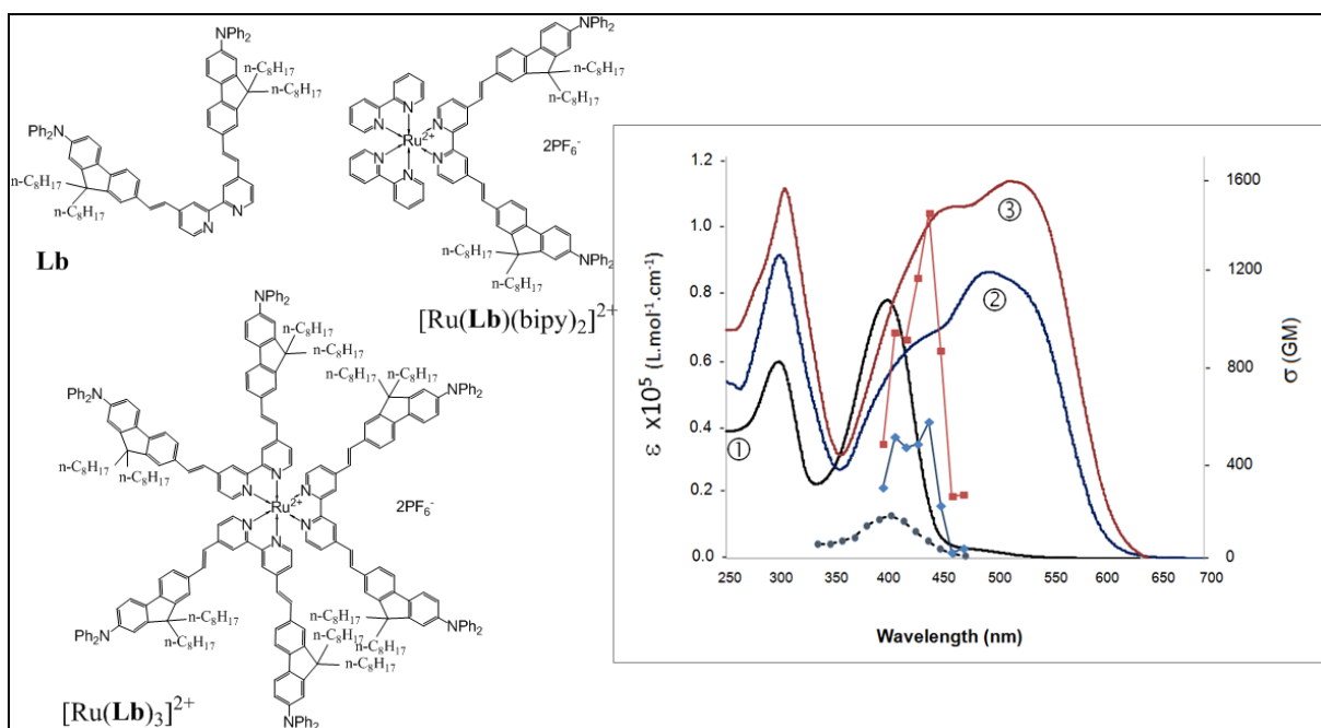
Figure 3. Left : Chemical structures of Lb , [\text{Ru}(\text{Lb})(\text{bipy})_2]^{2+} , [\text{Ru}(\text{Lb})_3]^{2+} . Right: 1PA and 2PA spectra for Lb (black curves; ①), [\text{Ru}(\text{Lb})(\text{bipy})_2]^{2+} (blue curves; ②), [\text{Ru}(\text{Lb})_3]^{2+} (red curves; ③), in \text{CH}_2\text{Cl}_2 ( 10^{-6} \text{ M} ).
