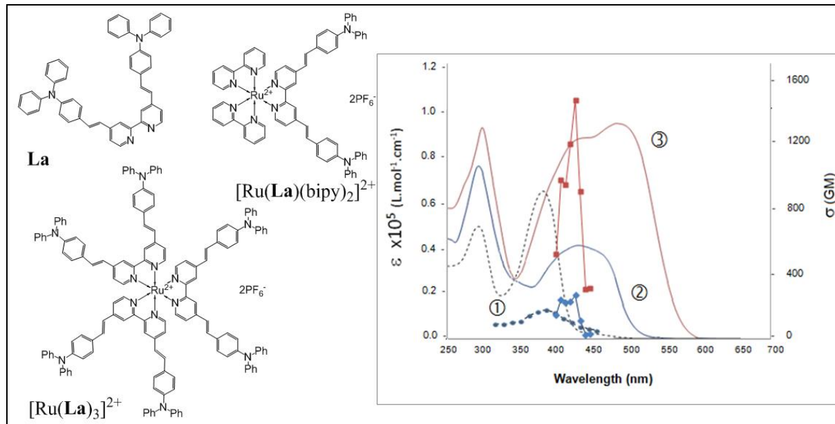
Figure 2. Left: Chemical structures of La , [\text{Ru}(\text{La})(\text{bipy})_2]^{2+} , [\text{Ru}(\text{La})_3]^{2+} . Right: 1PA and 2PA spectra for La (dotted curves; ①), [\text{Ru}(\text{La})(\text{bipy})_2]^{2+} (blue curves; ②), [\text{Ru}(\text{La})_3]^{2+} (red curves; ③), in \text{CH}_2\text{Cl}_2 ( 10^{-6} M).
