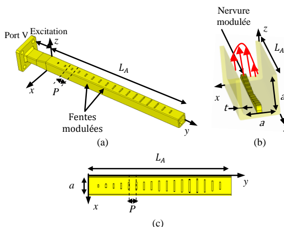
Figure 1. Structure de l'antenne (a) vue globale, (b) vue interne, (c) vue du dessus (30GHz, a = 6 mm, P = 4 mm, L_A = 10.8\lambda , t = 1 mm).
