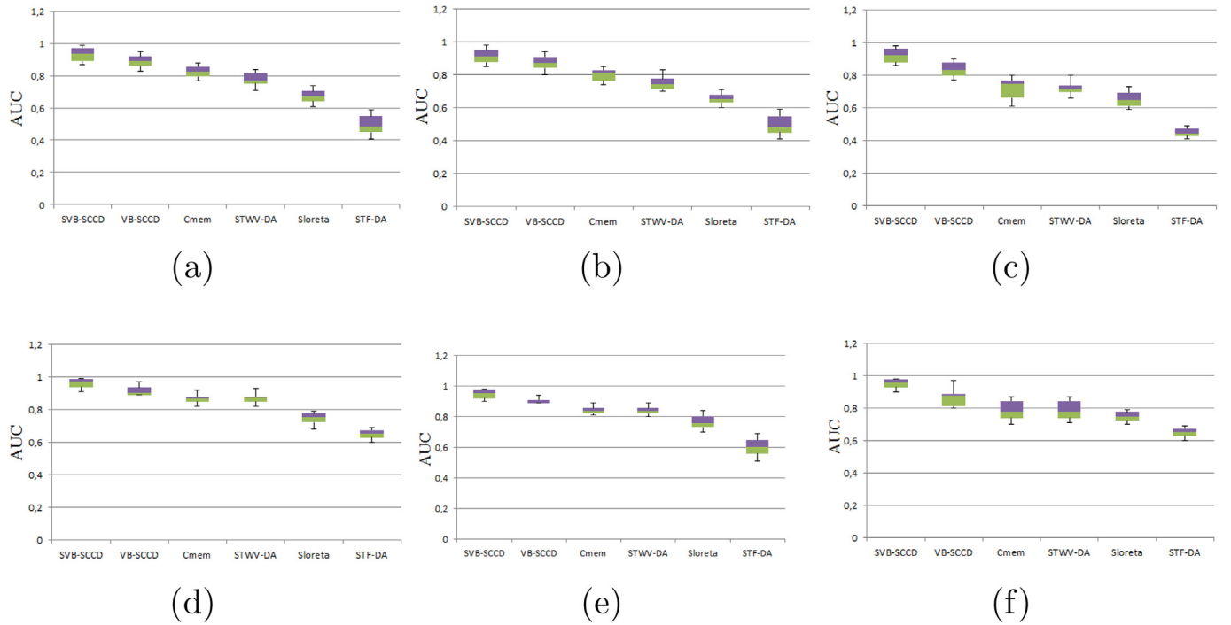
Fig. 1. AUC obtained for different methods applied to raw EHG data (up) and to spatially prewhitened EHG data (down) for three different scenarios composed of two patches with large distance (left), patches with medium distance (center), and patches small distance (right).
