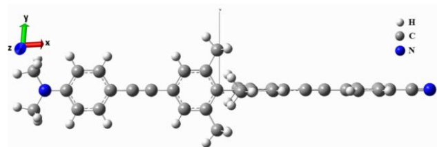
Figure 9. Optimized structure of TBP in gas phase.
