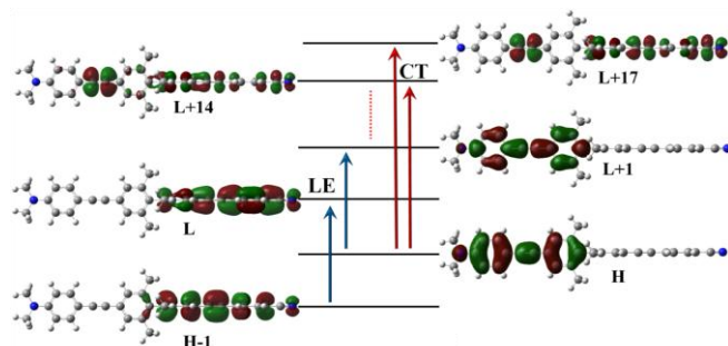
Figure 11. Frontier Molecular Orbitals of TBP obtained with ZINDO calculations showing the LE/CT transitions. Blue arrow indicates LE transition and red arrow indicates CT transition.
