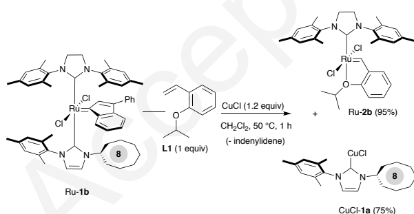
Scheme 3 Transmetalation process between Cu(I)Cl and mixed NHC Ru- 1b complex
