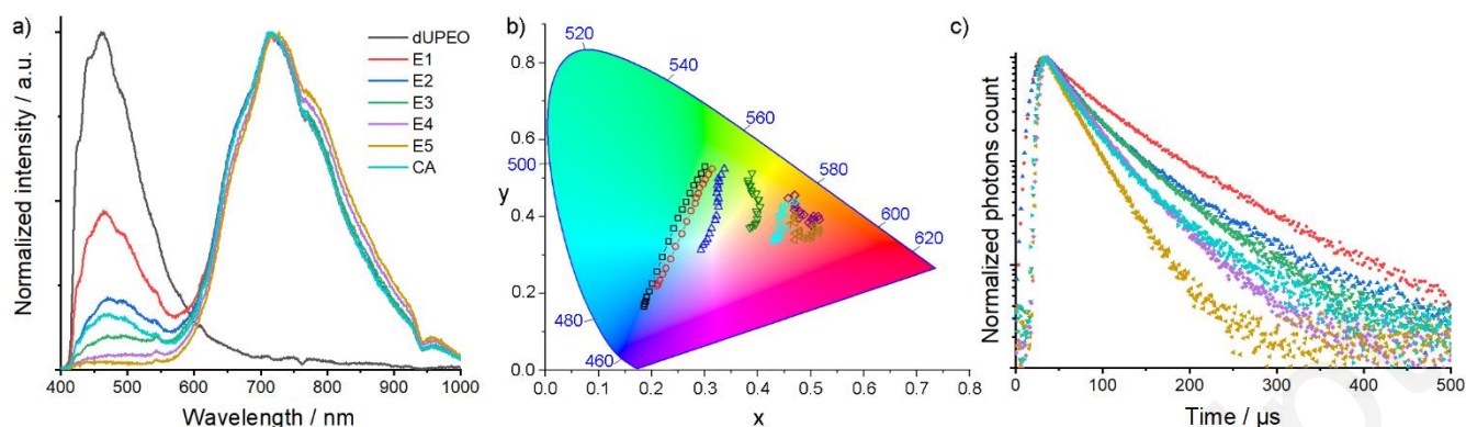
Figure 2. a) Normalized emission spectra of hybrid materials irradiated between 350–380 nm; b) CIE 1938 diagram coordinates for excitation ranging from 365 up to 450 nm: dUPEO (black), E1 (red), E2 (blue), E3 (green), E4 (purple), E5 (maroon) and CA (cyan); c) phosphorescence emission decay profiles recorded in the metal cluster emission range (662–798 nm).
