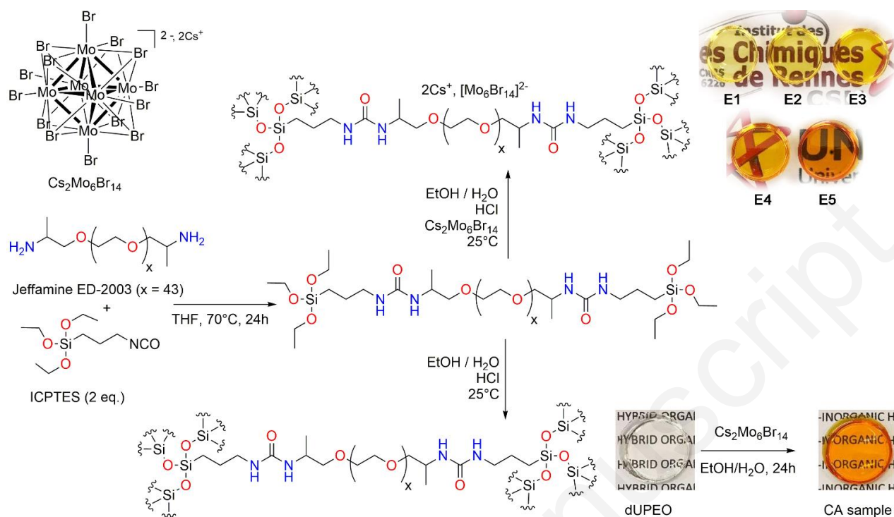
Figure 1. Structure of octahedral \text{Cs}_2\text{Mo}_6\text{Br}_{14} metal cluster compound ( 1 ), diureasil PEO (dUPEO) hybrid sol and synthetic schemes for the preparation of unloaded and loaded dUPEO xerogel containing 1 .
