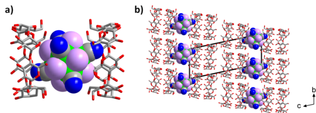
Figure 4: Views of the structural arrangement in the series K_4\{[Re_6Q_8(CN)_6]@(\beta-CD)_2\} \cdot 2(\beta-CD) \cdot nH_2O with Q = S ( Re_6S_8@β-CD ), Se ( Re_6Se_8@β-CD ) and Te ( Re_6Te_8@β-CD ). a) View of the rhenium cluster partially embedded within two \beta -CDs exposing their primary faces. b) View of the unit cell and the stacking of the supramolecular sheet along the perpendicular direction to the bc plane.
