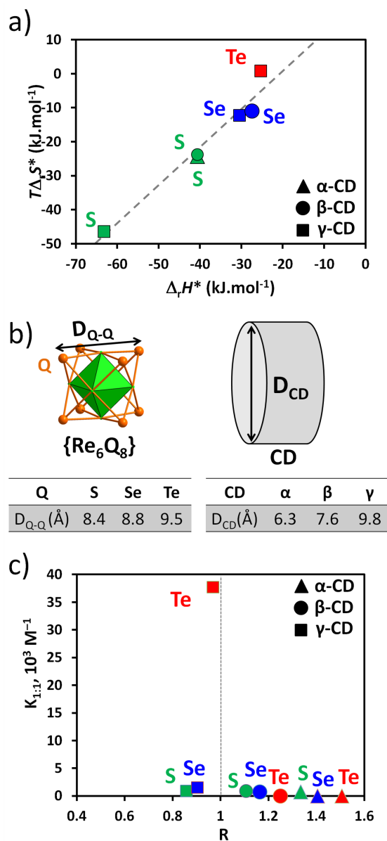
Figure 7. a) Enthalpy-entropy compensation plot for 1:1 cyclodextrin complexes with [\text{Re}_6\text{Q}_8(\text{CN})_6]^{4+} . b) Schematic representation showing the structural parameters used for the calculation of the host-guest structural fitting parameter R determined from the following equation: R = D_{Q-Q}/D_{CD} . c) Evolution of the one-site binding constant as a function of host-guest fitting parameter R .
