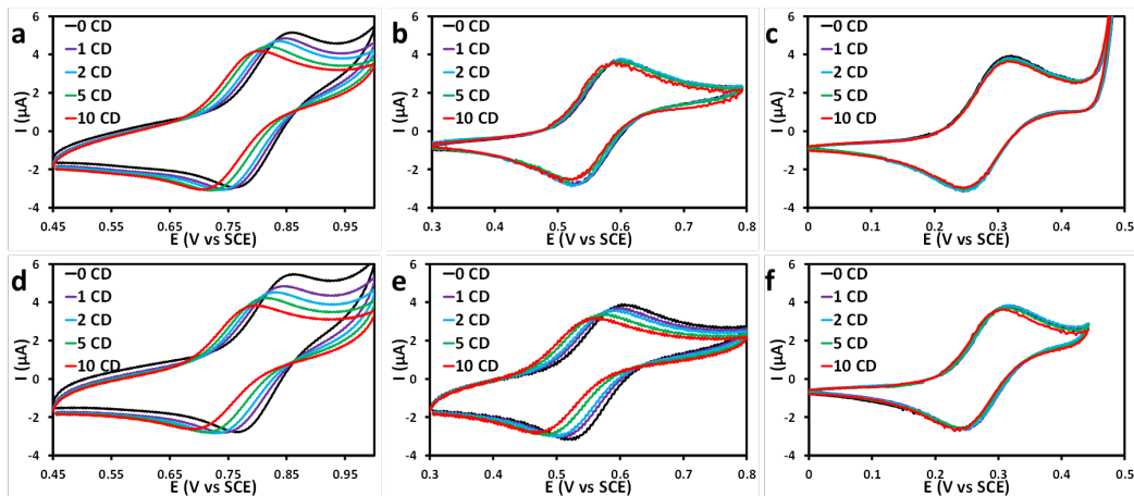
Figure 8: Cyclic voltammetry of the [\text{Re}_6\text{Q}_8(\text{CN})_6]^{4-} anions ( 0.5 \text{ mmol.L}^{-1} , 2.5 \text{ mmol.L}^{-1} \text{HClO}_4 aqueous solution, glassy carbon working electrode, scan rate 50 \text{ mV.s}^{-1} ) in the presence of increasing amounts of \alpha -CD (Q = S (a), Se (b) or Te (c)) or \beta -CD (Q = S (d), Se (e) or Te (f)).
