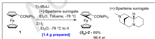
Scheme 3 Enantioselective synthesis of compound ( S p )- 2 .
