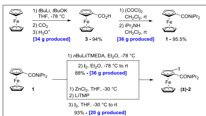
Scheme 2 Column chromatography-free multi-gram synthesis of compound ( ± )- 2 .
