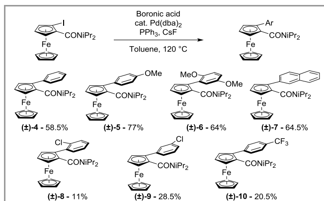
Scheme 4 Suzuki-Miyaura cross-coupling between ( ± )- 2 and various boronic acids.
