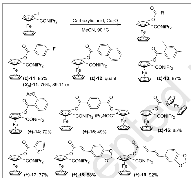
Scheme 5 Ullmann-type cross-coupling between ( ± )- 2 or ( S P )- 2 and various carboxylic acids.
