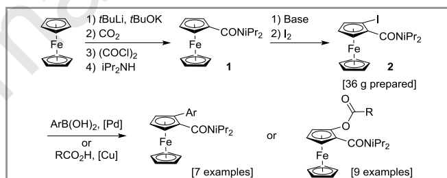
Scheme 1 Gram-scale synthesis of ( ± )- and ( S p )- 2 and their further functionalization.
