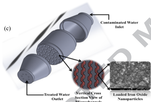
Fig. 1. (a) Geometry representation (in mm) (b) Actual 3D image and (c) Sectional view of loaded nanoparticles of the microchannel device
