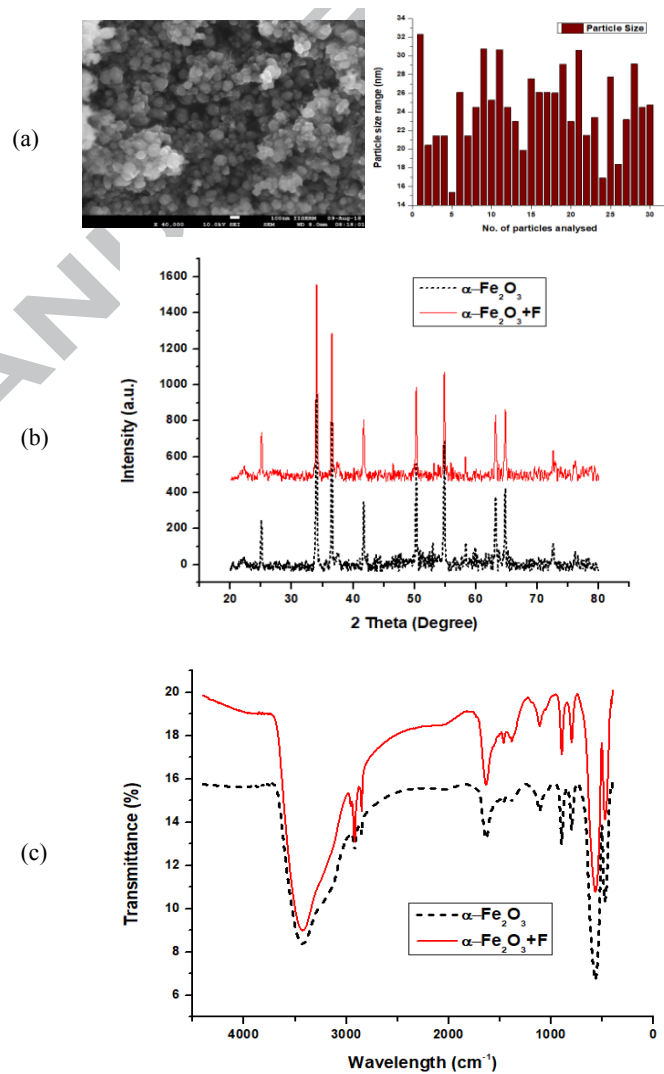
Fig. 3. (a) FESEM image and particle size of nanoparticles (b) XRD and (c) FTIR characterization of iron oxide before and after fluoride adsorption
