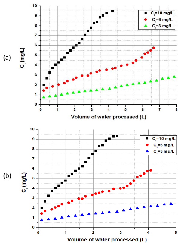
Fig. 4. (a) and (b) shows experimental bends representing adsorption of fluoride onto iron oxide at varying fluoride concentrations (3, 6 and 10 mg/L) for adsorbent dosage= 4.0 g and 3.0 g respectively at temperature = 25 °C )
