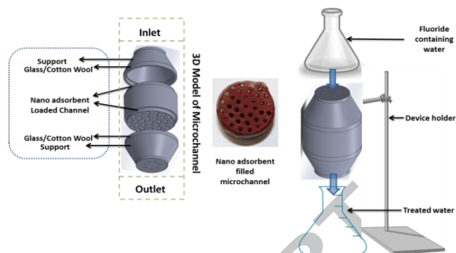
Fig. 2. Process flow system setup for the removal of fluoride from water
