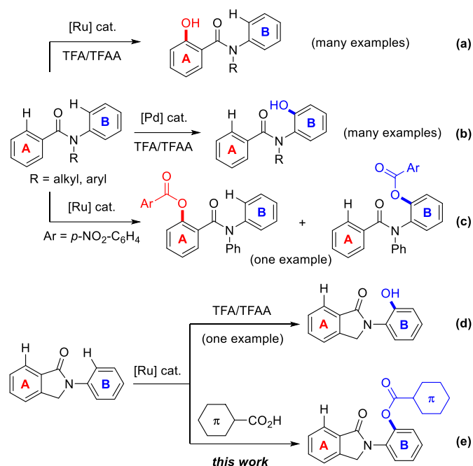
Fig. 1 State-of-the-art for the transition metal-catalysed C-H bond hydro/benzoylations of N -substituted phenylbenzamides as weak directing groups (a-d) and present work (e).
