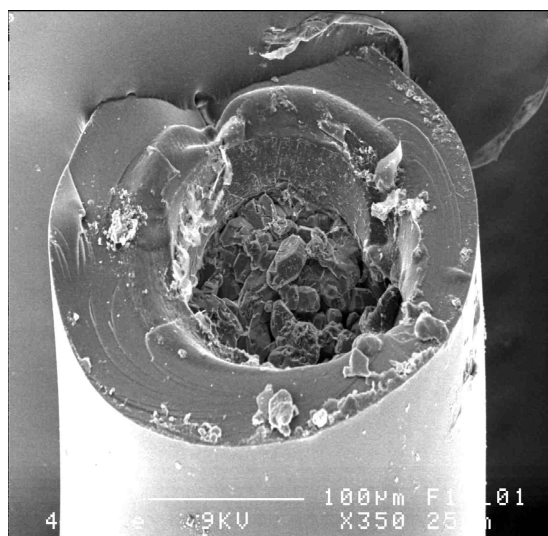
Figure 10. Harsh etching of unprotected end of silica cladding in fluorinated environment (H SOF)
