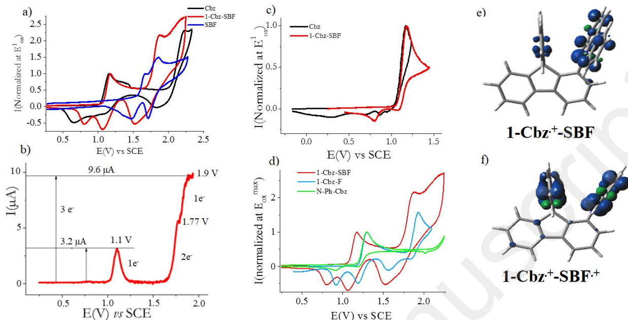
Figure 3. a) CVs recorded at 100 \text{ mV s}^{-1} (potential range of 0.2/2.2 V) in \text{CH}_2\text{Cl}_2/[\text{Bu}_4\text{N}][\text{PF}_6] 0.2 M in the presence of 1-Cbz-SBF (red line), SBF (blue line), and Cbz (black line). b) Differential pulse voltammometry of 1-Cbz-SBF . c) CVs recorded at 100 \text{ mV s}^{-1} (potential range of -0.2/1.45 V) in \text{CH}_2\text{Cl}_2/[\text{Bu}_4\text{N}][\text{PF}_6] 0.2 M in the presence of 1-Cbz-SBF (red line) and Cbz (black line). d) CVs recorded at 100 \text{ mV s}^{-1} (potential range of 0.2/2.25 V) in \text{CH}_2\text{Cl}_2/[\text{Bu}_4\text{N}][\text{PF}_6] 0.2 M in the presence of 1-Cbz-SBF (red line), N-Ph-Cbz (green line) and 1-Cbz-F (sky blue line). Intensity is normalized at E_{\text{ox}}^1 for all the compounds. Spin densities of (e) the cation radical and the bis radical cation (f) of 1-Cbz-SBF (isovalue = 0.004, cam-b3lyp/6-31g(d)).
