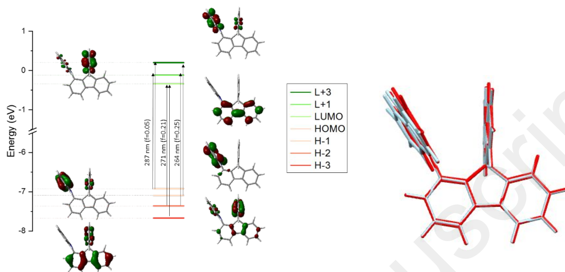
Figure 7. Left: Representation of the energy levels and the main molecular orbitals involved in the electronic transitions of 1-Cbz-SBF obtained by TD-DFT CAM-B3LYP/6-311+G(d,p), shown with an isovalue of 0.04 [ e \text{ bohr}^{-3} ] ^{1/2} . For clarity purposes, only the major contributions (>10%) of each transition is shown (see SI for details). Right: Superposition of optimized geometries of S_0 (ground state, light blue) and S_1 (first singlet excited state, red).
