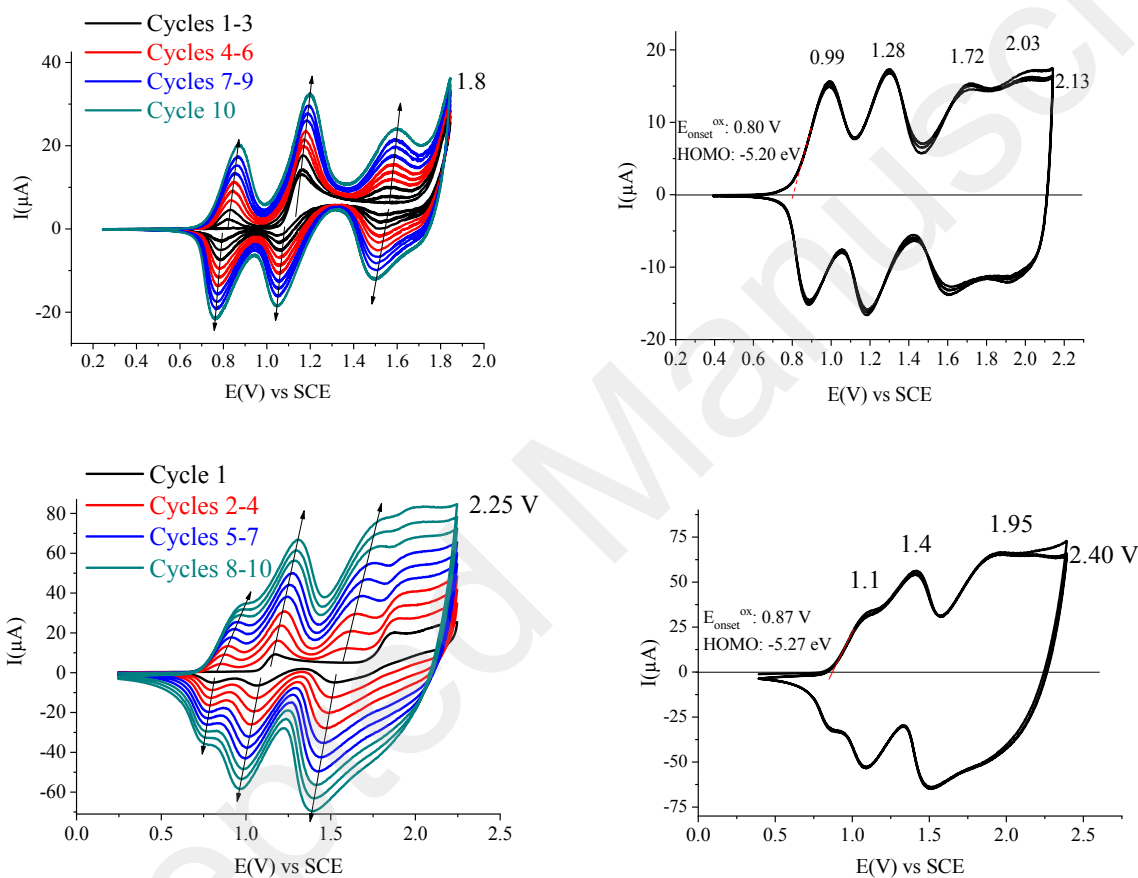
Figure 4. Left: CV ( 100 \text{ mV s}^{-1} , \text{CH}_2\text{Cl}_2/[\text{Bu}_4\text{N}][\text{PF}_6] 0.2 M) in the presence of 1-Cbz-SBF , 2.7 \times 10^{-3} M, potential range of the ten successive cycles : 0.2-1.8 V (top) or 0.2-2.25 V (bottom), platinum disk working electrode. Right: CV ( 100 \text{ mV s}^{-1} , \text{CH}_2\text{Cl}_2/[\text{Bu}_4\text{N}][\text{PF}_6] 0.2 M) free of any electroactive species, potential limit of the three successive cycles: 0.2-2.13 V (top) or 0.2-2.40 V (bottom), platinum disk working electrode modified by the deposits obtained along the ten cycles in presence of 1-Cbz-SBF .
