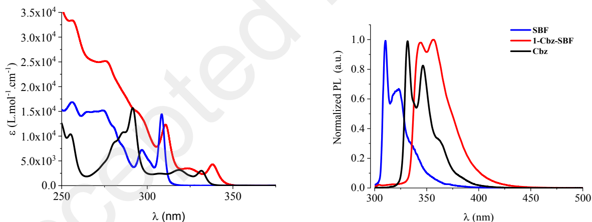
Figure 6. Absorption spectra (left) and normalized emission spectra (right) of 1-Cbz-SBF (red line), SBF (blue line) and Cbz (black line) in cyclohexane at room temperature.
