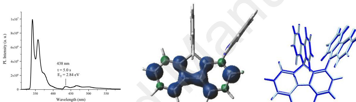
Figure 8. Left: emission spectrum of 1-Cbz-SBF at 77 K (2-Me-THF, \lambda_{exc} = 300 \text{ nm} ). Middle: Spin density of triplet of 1-Cbz-SBF (isovalue= 0.004). Right: Superposition of optimized geometries: S_0 (ground state, light blue) and T_1 (first triplet excited state, blue)
