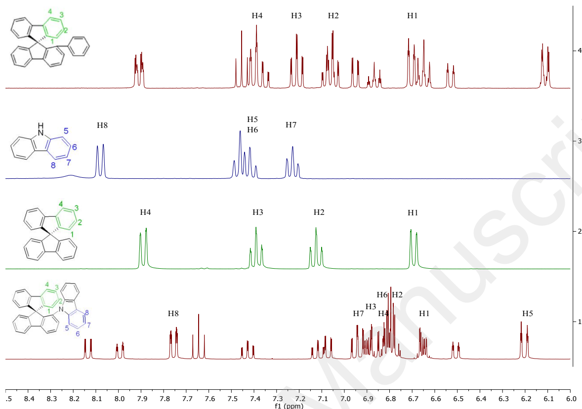
Figure 1. 1 H NMR spectra in CD 2 Cl 2 of 1-Ph-SBF , Cbz , SBF and 1-Cbz-SBF (From top to bottom respectively).
