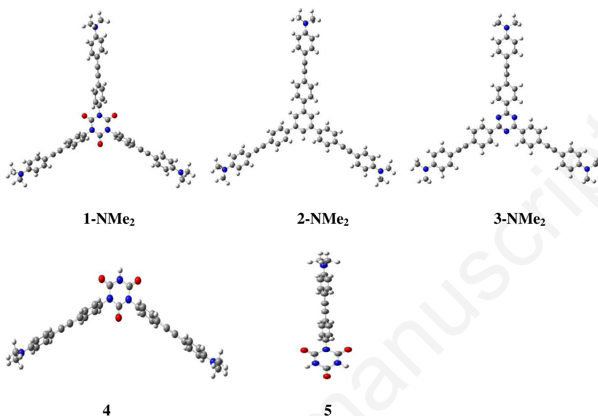
Fig. 1 Optimized geometries in \text{CH}_2\text{Cl}_2 of the derivatives under study.
