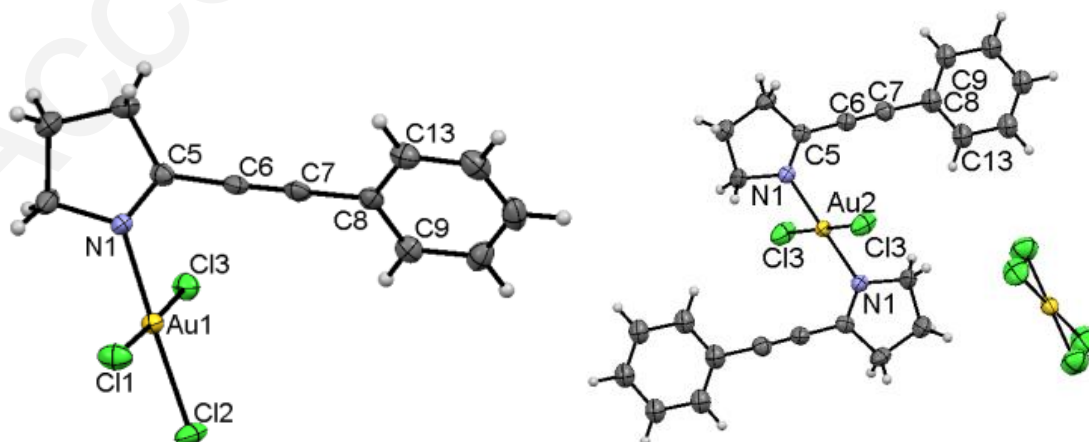
Scheme 7. Synthesis of complexes ML and ML2
