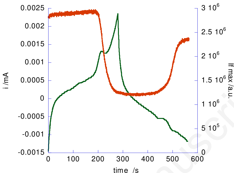
Figure 5. Fluorescence intensity (red trace, right scale) and electrochemical current (green trace, left scale) for 1 in CH 2 Cl 2 / [NBu 4 ][PF 6 ] (0.1 M) as functions of time upon potential linear scan from 0 V to 1.4 V and back to 0 V (scan rate : 2 mV/s). Recorded in a thin layer spectroelectrochemical cell coupled to a spectrofluorimeter (excitation 420 nm).
