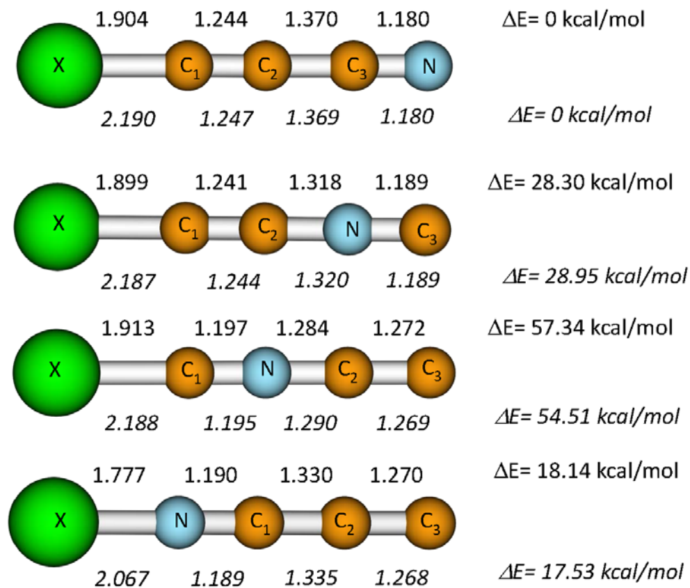
Figure 1. Equilibrium geometries and relative energies (ZPE corrections are included) of the equilibrium structures for the different MC_3N ( M=Li,Na ) isomers obtained at the MP2/aug-cc-pVTZ and the CCSD(T)/aug-cc-pVTZ//MP2/aug-cc-pVTZ levels respectively. Distances are given in Ångstroms. Upper values are for LiC_3N species, whereas lower values (in Italics ) correspond to NaC_3N isomers.
