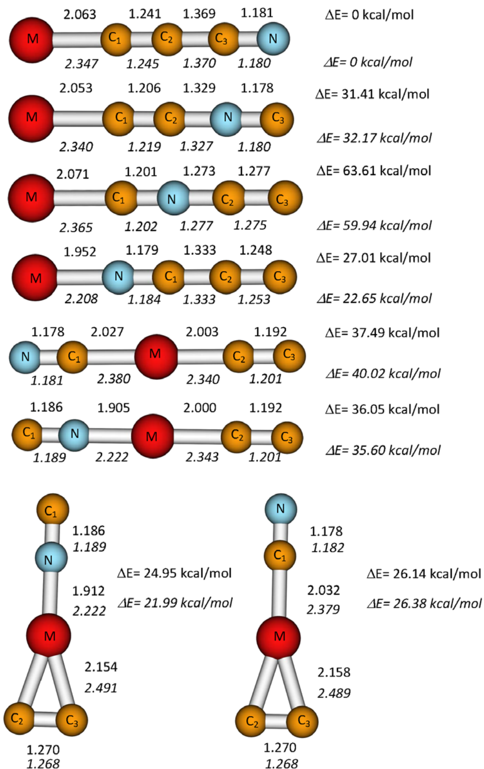
Figure 4. Equilibrium geometries and relative energies (ZPE corrections are included) for the different MC 3 N (M=Mg,Ca) isomers obtained at the MP2/aug-cc-pVTZ and the CCSD(T)/aug-cc-pVTZ//MP2/aug-cc-pVTZ levels respectively. Distances are given in Ångstroms. Upper values are for MgC 3 N species, whereas lower values (in Italics) correspond to CaC 3 N isomers.
