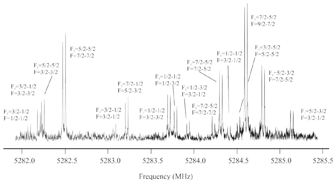
Figure 3. Central section of the J = 2-1 rotational transition of NaCCCN. The nuclear quadrupole coupling hyperfine structure arising from both from both {}^{23}\text{Na} ( I=3/2 ) and {}^{14}\text{N} ( I=1 ) nuclei is clearly resolved. Each hyperfine component is labeled with the corresponding values of F_1' , F' \leftarrow F_1'' , F'' quantum numbers.
