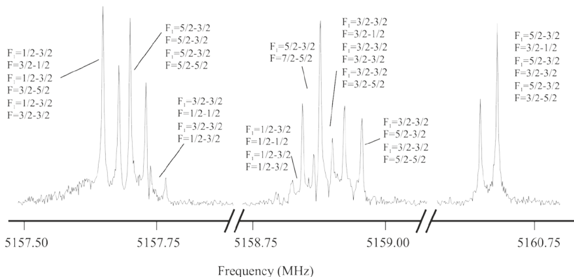
Figure 2. Spectrum of a section of the J = 1-0 rotational transition of LiCCCN near 5.2 GHz showing the multiple hyperfine components arising from both {}^7\text{Li} ( I=3/2 ) and {}^{14}\text{N} ( I=1 ) nuclei. The coaxial arrangement of the adiabatic expansion and the resonator axis produces an instrumental Doppler doubling. The resonances frequencies are calculated as the average of the two Doppler components. Each hyperfine component is labeled with the corresponding values of F_1' , F' \leftarrow F_1'' , F'' quantum numbers.
