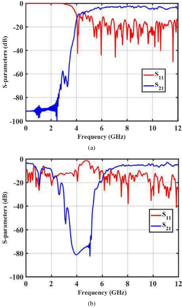
Fig. 6. Simulated S_{11} and S_{21} magnitude of the slotted antenna. (a) Plasma OFF. (b) Plasma ON.
